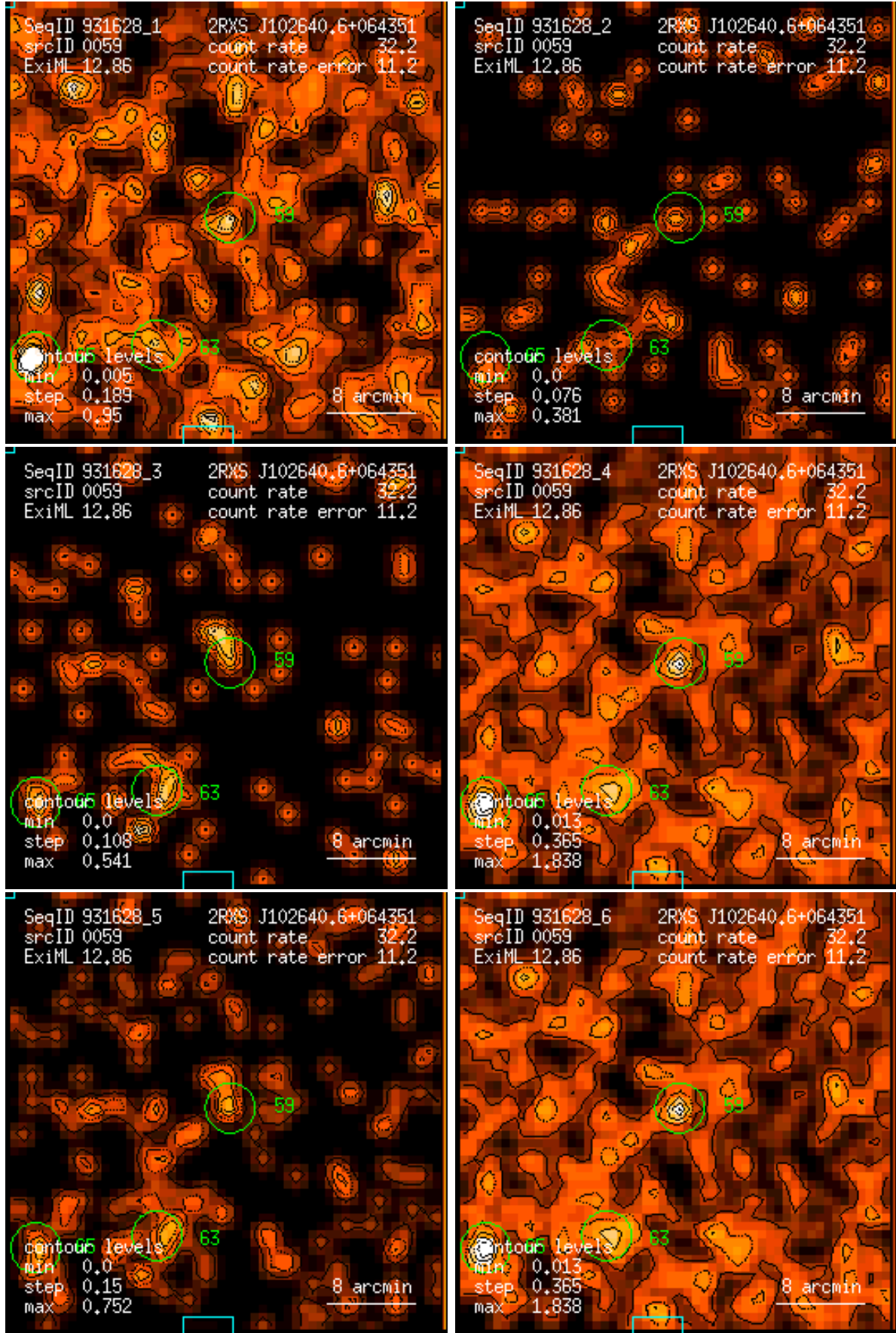
Figure 59: RASS 931628: detection 0059: band rate images, Gaussian filter: (1) PSPC channels 11 – 41, (2) 52 – 90, (3) 91 – 201, (4) 11 – 235, (5) 52 – 201, (6) 11 – 201. Broad band rates in counts/ks. Band rate contour levels in counts/ks/arcmin 2 .
