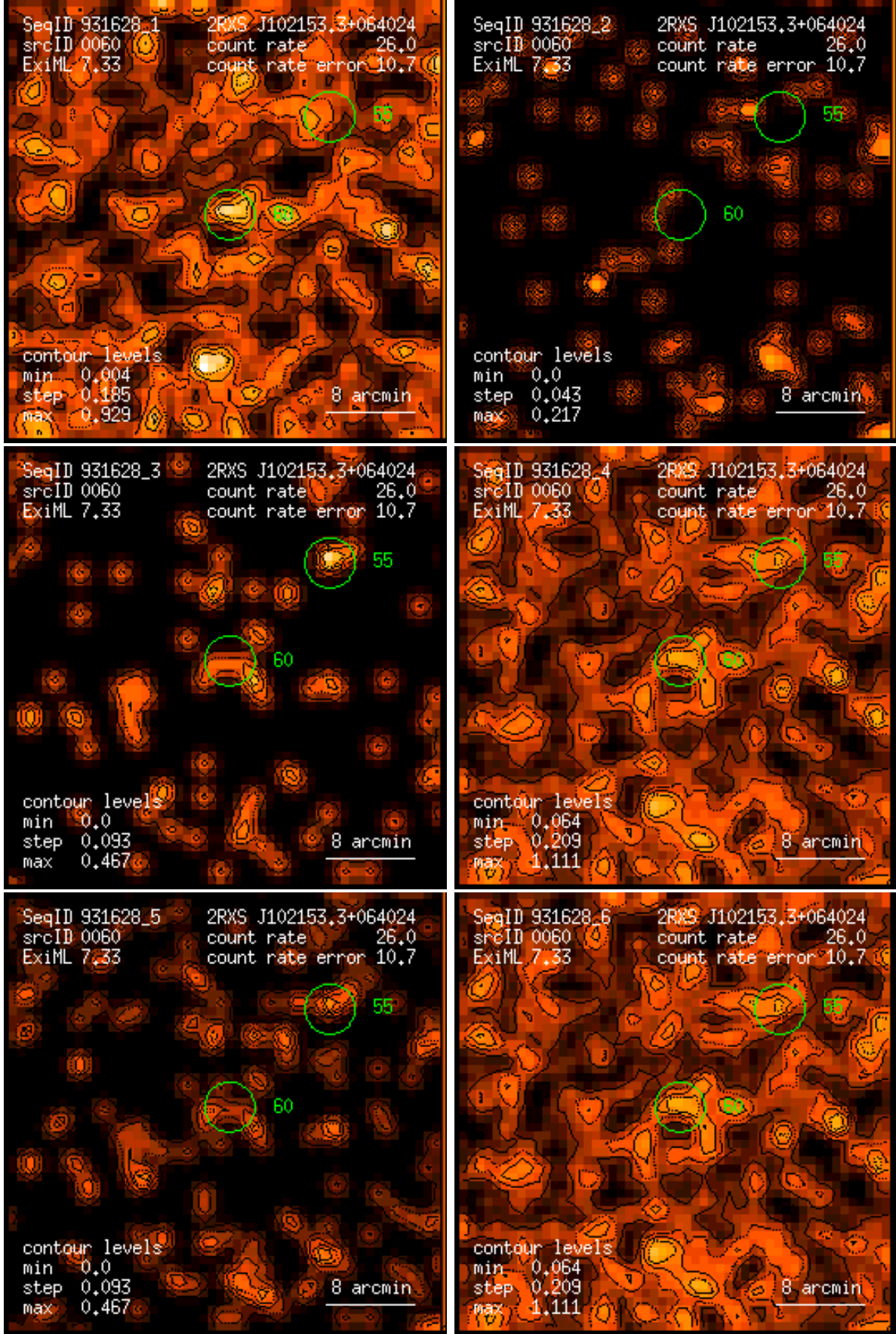
Figure 60: RASS 931628: detection 0060: band rate images, Gaussian filter: (1) PSPC channels 11 – 41, (2) 52 – 90, (3) 91 – 201, (4) 11 – 235, (5) 52 – 201, (6) 11 – 201. Broad band rates in counts/ks. Band rate contour levels in counts/ks/arcmin 2 .
