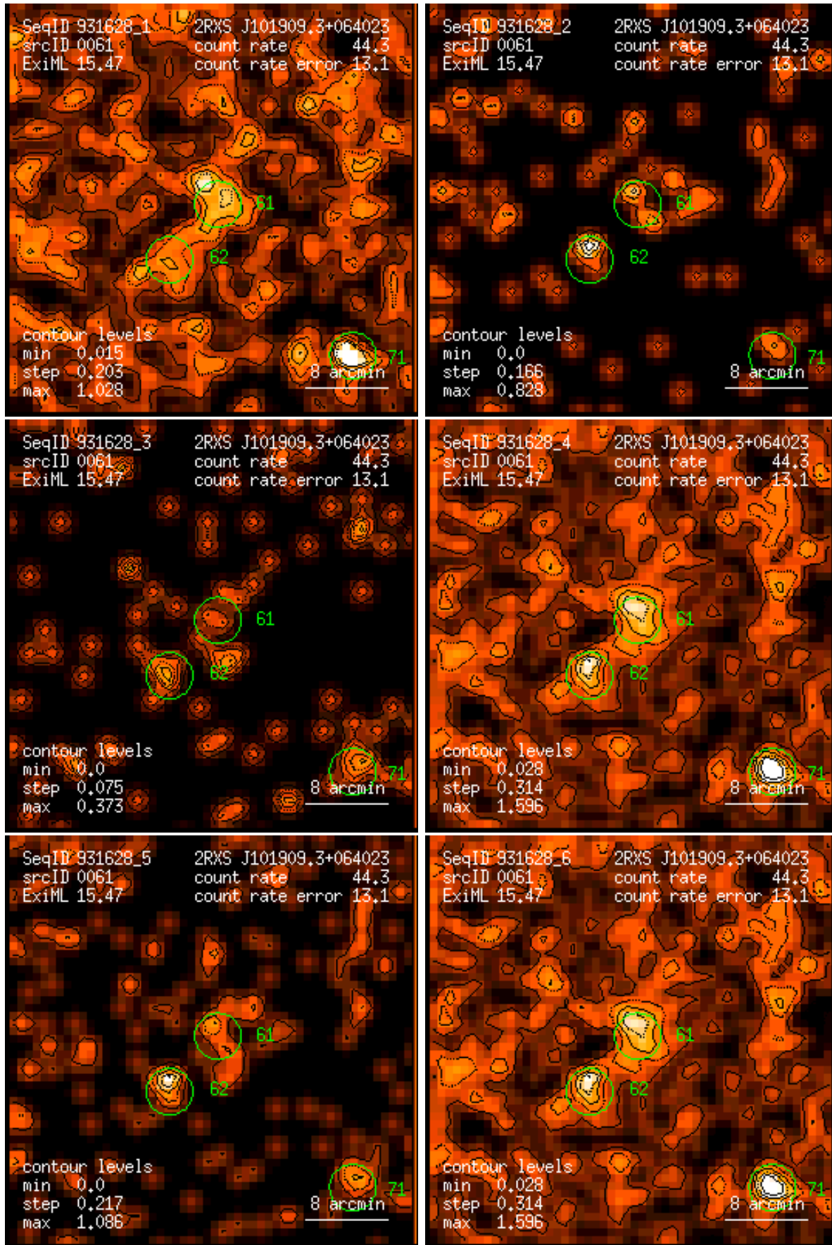
Figure 61: RASS 931628: detection 0061: band rate images, Gaussian filter: (1) PSPC channels 11 – 41, (2) 52 – 90, (3) 91 – 201, (4) 11 – 235, (5) 52 – 201, (6) 11 – 201. Broad band rates in counts/ks. Band rate contour levels in counts/ks/arcmin 2 .
