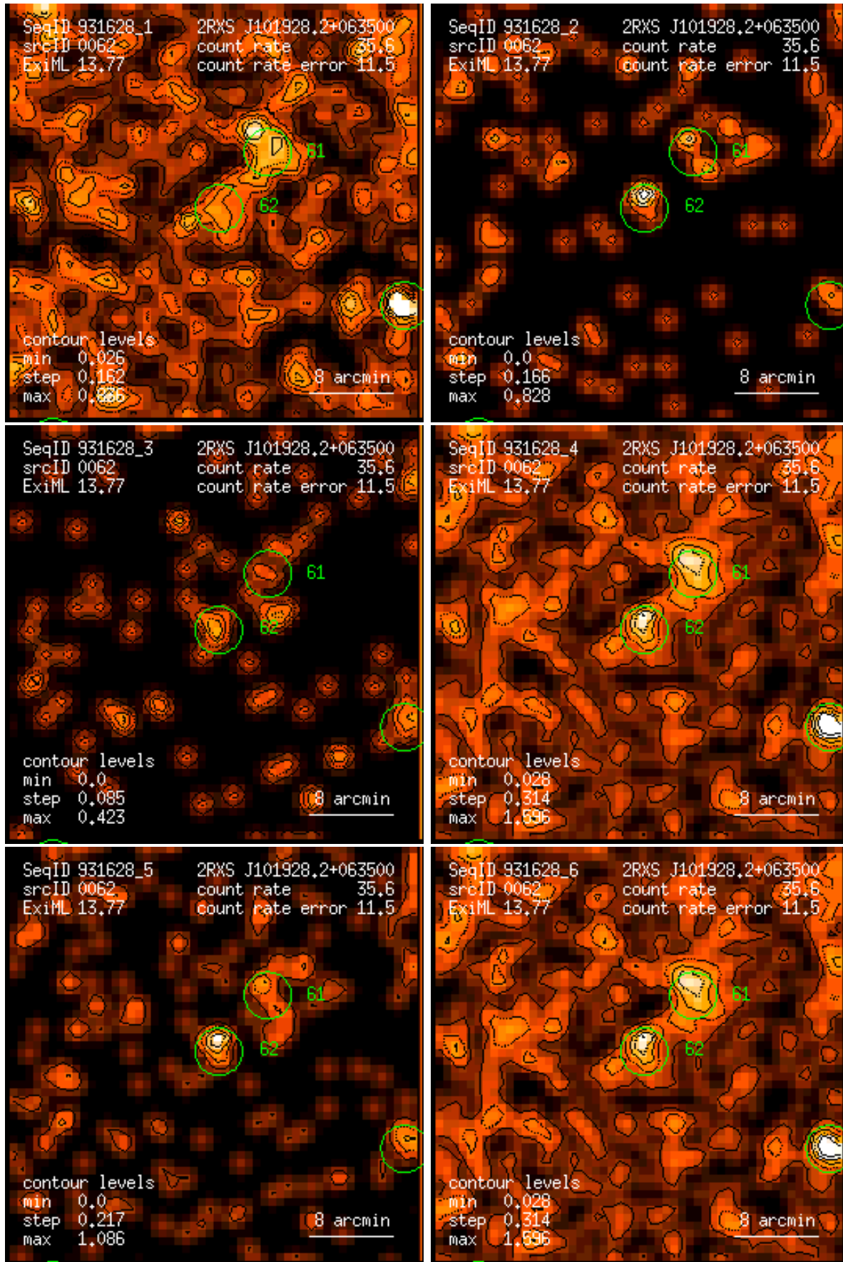
Figure 62: RASS 931628: detection 0062: band rate images, Gaussian filter: (1) PSPC channels 11 – 41, (2) 52 – 90, (3) 91 – 201, (4) 11 – 235, (5) 52 – 201, (6) 11 – 201. Broad band rates in counts/ks. Band rate contour levels in counts/ks/arcmin 2 .
