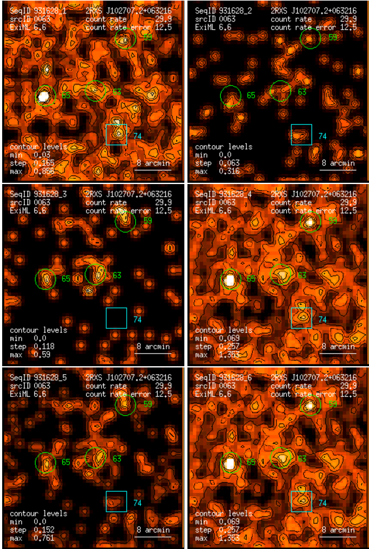
Figure 63: RASS 931628: detection 0063: band rate images, Gaussian filter: (1) PSPC channels 11 – 41, (2) 52 – 90, (3) 91 – 201, (4) 11 – 235, (5) 52 – 201, (6) 11 – 201. Broad band rates in counts/ks. Band rate contour levels in counts/ks/arcmin 2 .
