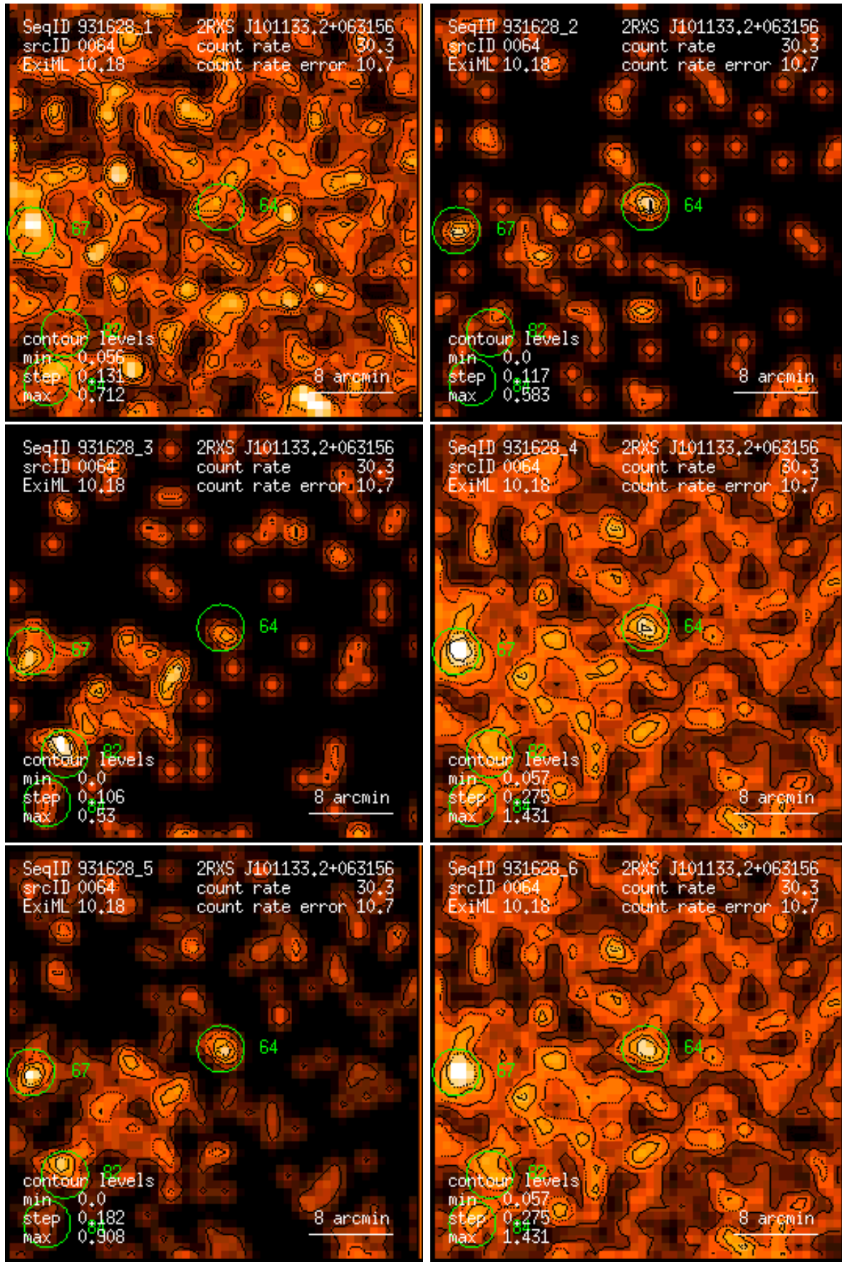
Figure 64: RASS 931628: detection 0064: band rate images, Gaussian filter: (1) PSPC channels 11 – 41, (2) 52 – 90, (3) 91 – 201, (4) 11 – 235, (5) 52 – 201, (6) 11 – 201. Broad band rates in counts/ks. Band rate contour levels in counts/ks/arcmin 2 .
