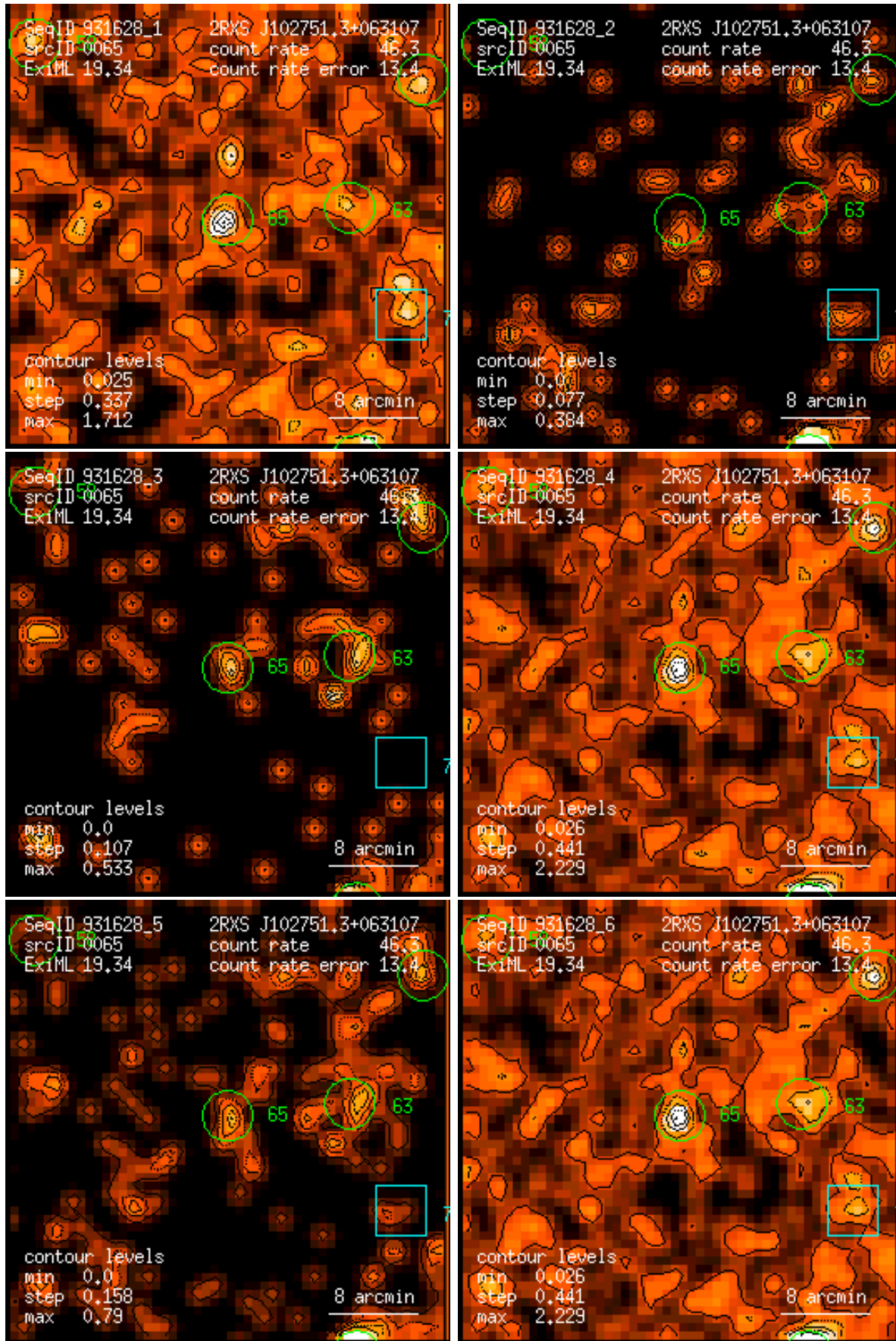
Figure 65: RASS 931628: detection 0065: band rate images, Gaussian filter: (1) PSPC channels 11 – 41, (2) 52 – 90, (3) 91 – 201, (4) 11 – 235, (5) 52 – 201, (6) 11 – 201. Broad band rates in counts/ks. Band rate contour levels in counts/ks/arcmin 2 .
