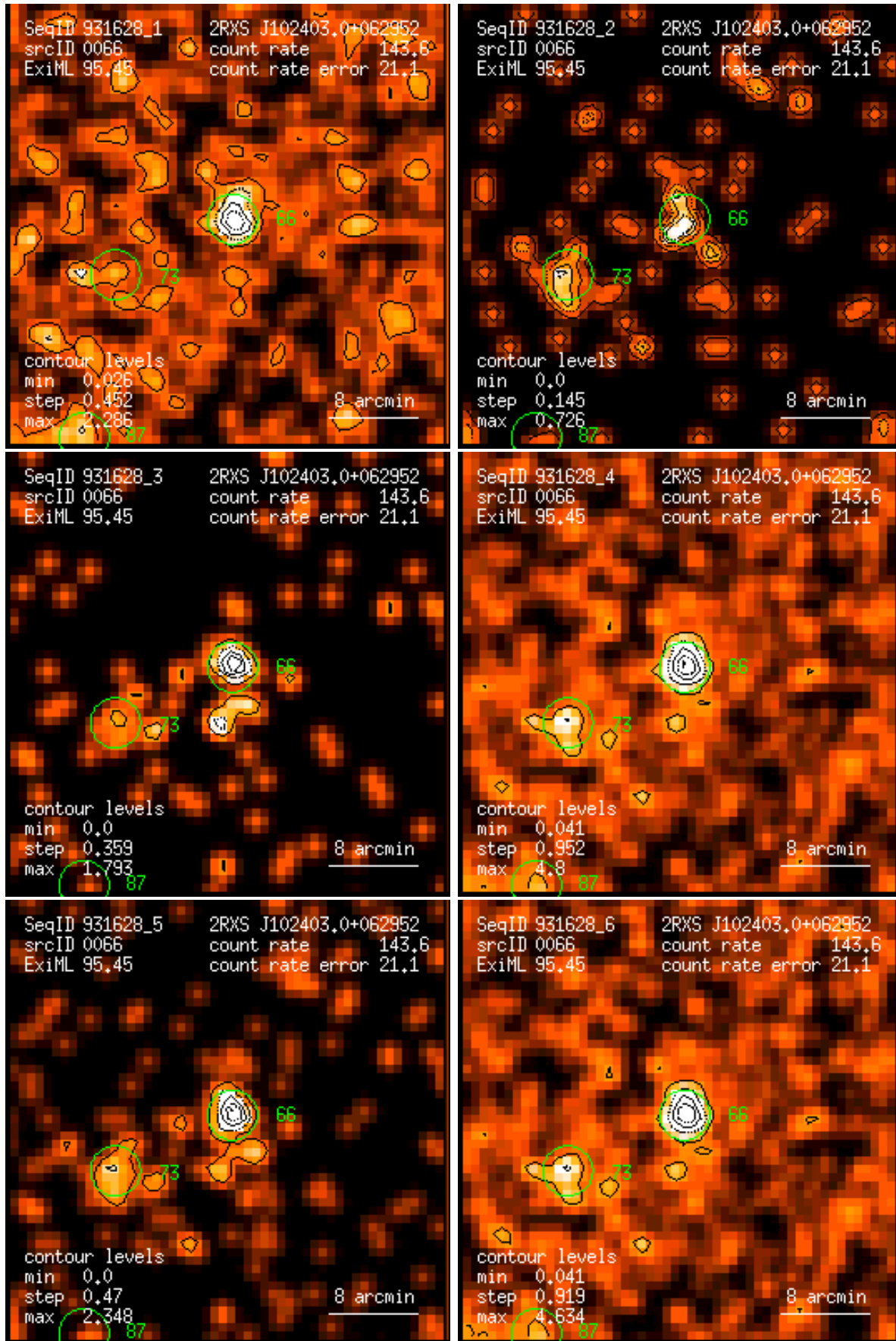
Figure 66: RASS 931628: detection 0066: band rate images, Gaussian filter: (1) PSPC channels 11 – 41, (2) 52 – 90, (3) 91 – 201, (4) 11 – 235, (5) 52 – 201, (6) 11 – 201. Broad band rates in counts/ks. Band rate contour levels in counts/ks/arcmin 2 .
