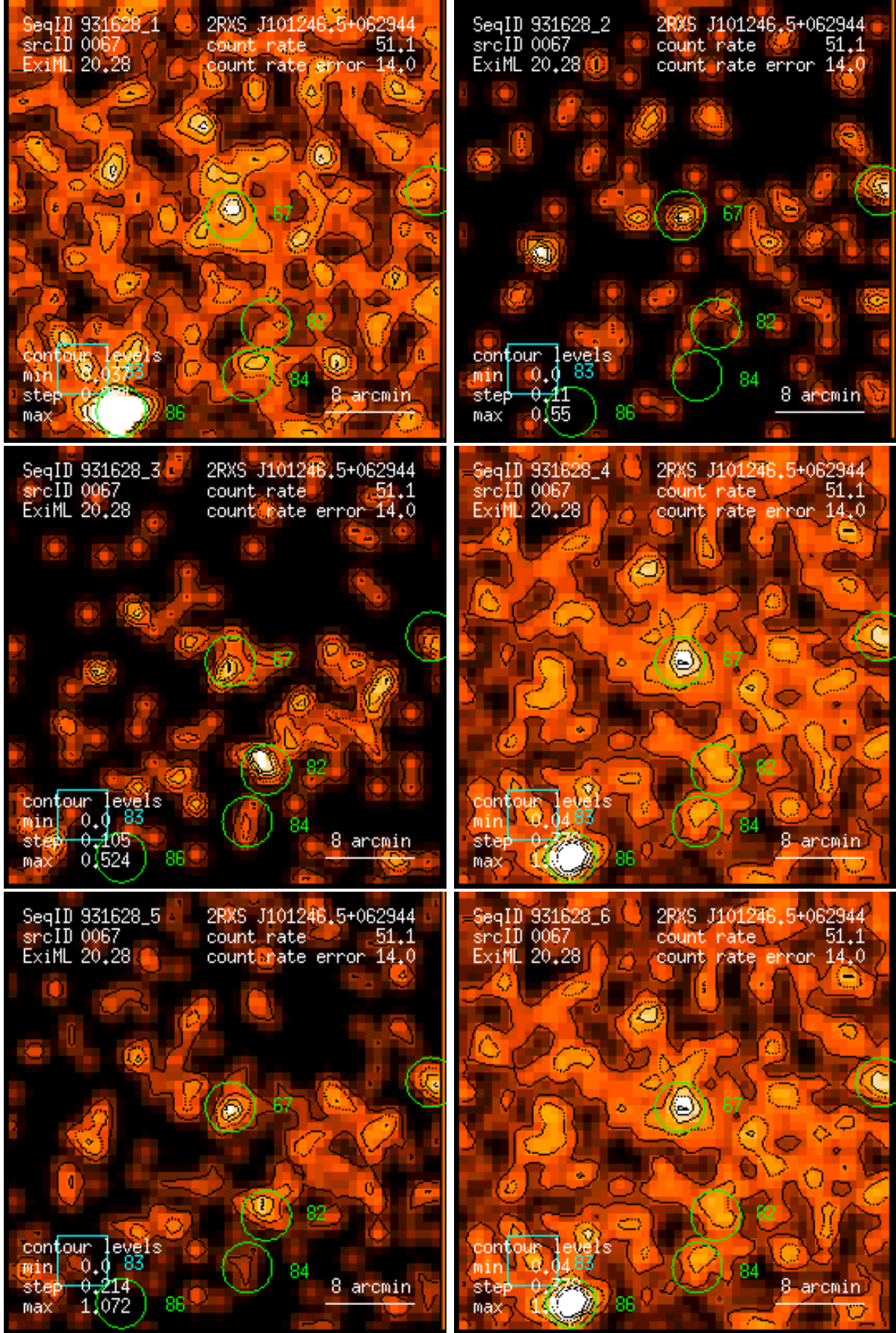
Figure 67: RASS 931628: detection 0067: band rate images, Gaussian filter: (1) PSPC channels 11 – 41, (2) 52 – 90, (3) 91 – 201, (4) 11 – 235, (5) 52 – 201, (6) 11 – 201. Broad band rates in counts/ks. Band rate contour levels in counts/ks/arcmin 2 .
