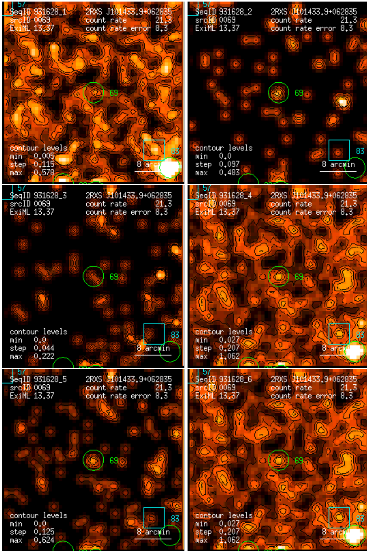
Figure 69: RASS 931628: detection 0069: band rate images, Gaussian filter: (1) PSPC channels 11 – 41, (2) 52 – 90, (3) 91 – 201, (4) 11 – 235, (5) 52 – 201, (6) 11 – 201. Broad band rates in counts/ks. Band rate contour levels in counts/ks/arcmin 2 .
