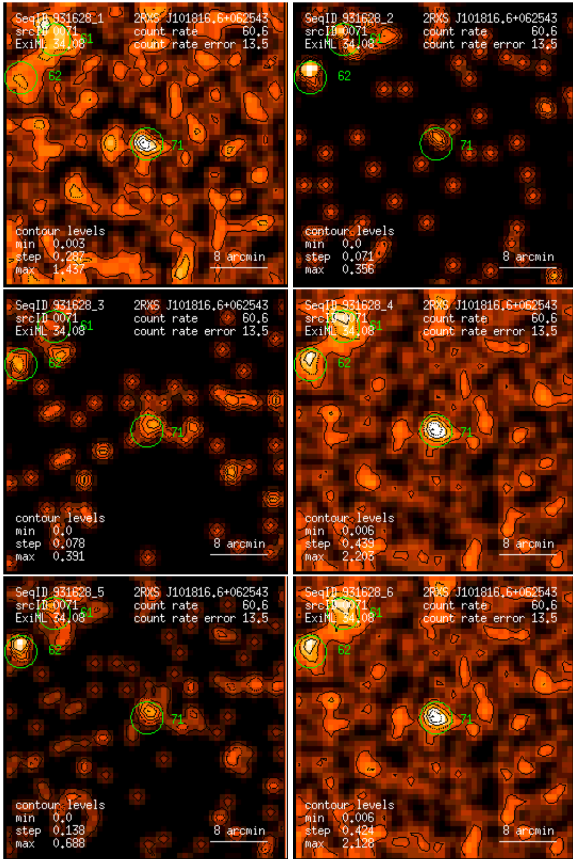
Figure 71: RASS 931628: detection 0071: band rate images, Gaussian filter: (1) PSPC channels 11 – 41, (2) 52 – 90, (3) 91 – 201, (4) 11 – 235, (5) 52 – 201, (6) 11 – 201. Broad band rates in counts/ks. Band rate contour levels in counts/ks/arcmin 2 .
