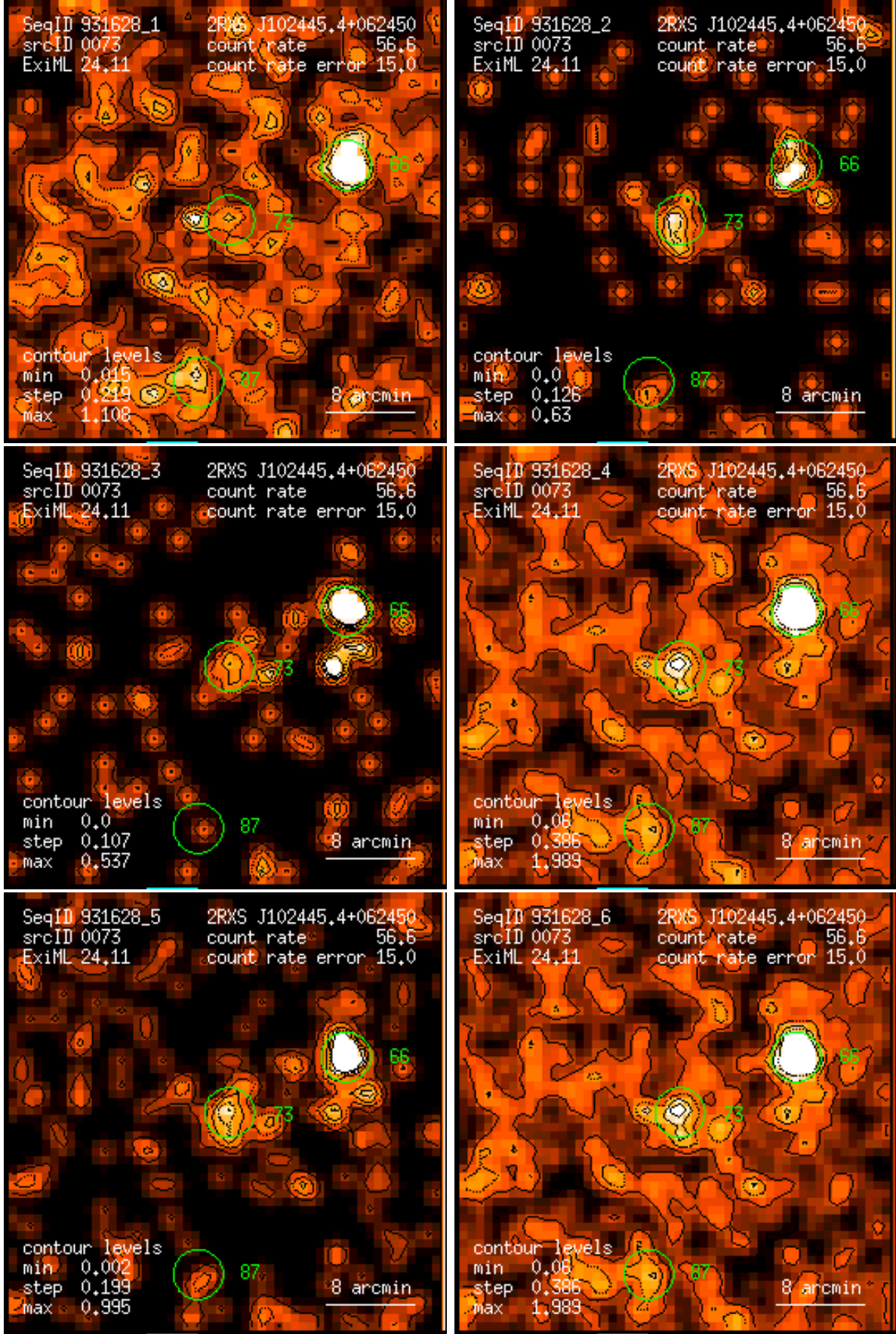
Figure 73: RASS 931628: detection 0073: band rate images, Gaussian filter: (1) PSPC channels 11 – 41, (2) 52 – 90, (3) 91 – 201, (4) 11 – 235, (5) 52 – 201, (6) 11 – 201. Broad band rates in counts/ks. Band rate contour levels in counts/ks/arcmin 2 .
