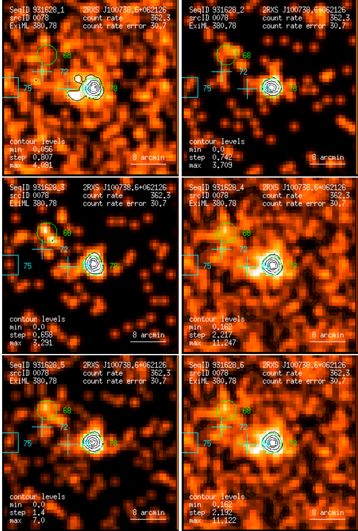
Figure 78: RASS 931628: detection 0078: band rate images, Gaussian filter: (1) PSPC channels 11 – 41, (2) 52 – 90, (3) 91 – 201, (4) 11 – 235, (5) 52 – 201, (6) 11 – 201. Broad band rates in counts/ks. Band rate contour levels in counts/ks/arcmin 2 .
