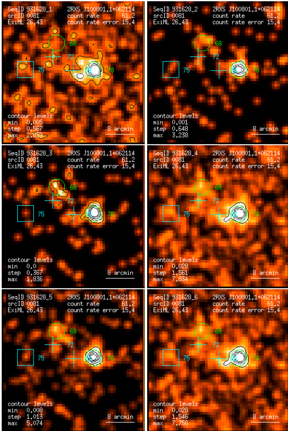
Figure 81: RASS 931628: detection 0081: band rate images, Gaussian filter: (1) PSPC channels 11 – 41, (2) 52 – 90, (3) 91 – 201, (4) 11 – 235, (5) 52 – 201, (6) 11 – 201. Broad band rates in counts/ks. Band rate contour levels in counts/ks/arcmin 2 .
