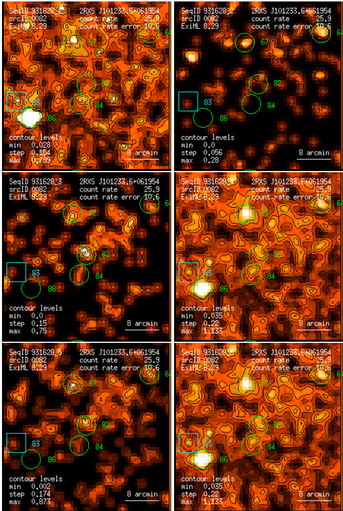
Figure 82: RASS 931628: detection 0082: band rate images, Gaussian filter: (1) PSPC channels 11 – 41, (2) 52 – 90, (3) 91 – 201, (4) 11 – 235, (5) 52 – 201, (6) 11 – 201. Broad band rates in counts/ks. Band rate contour levels in counts/ks/arcmin 2 .
