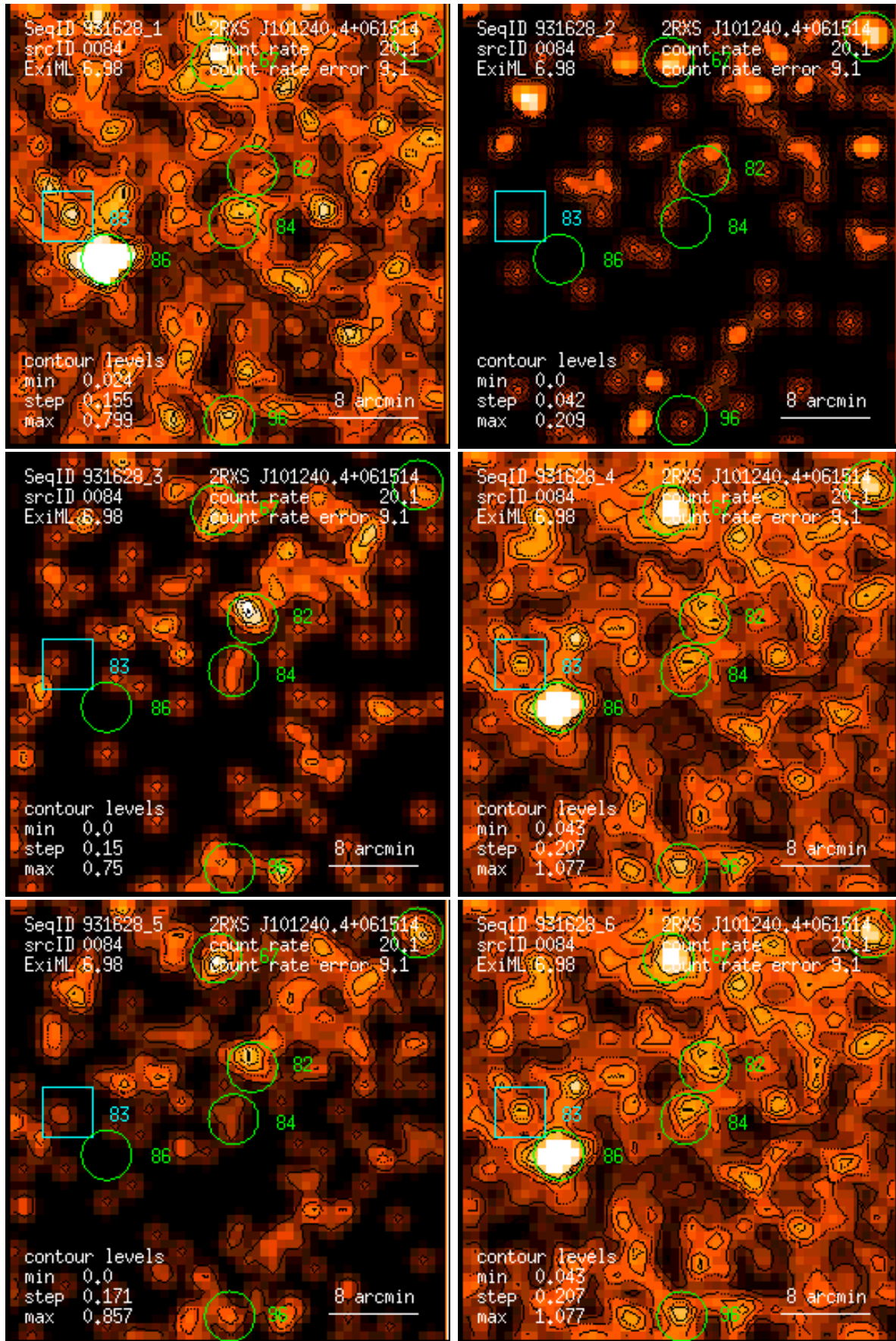
Figure 84: RASS 931628: detection 0084: band rate images, Gaussian filter: (1) PSPC channels 11 – 41, (2) 52 – 90, (3) 91 – 201, (4) 11 – 235, (5) 52 – 201, (6) 11 – 201. Broad band rates in counts/ks. Band rate contour levels in counts/ks/arcmin 2 .
