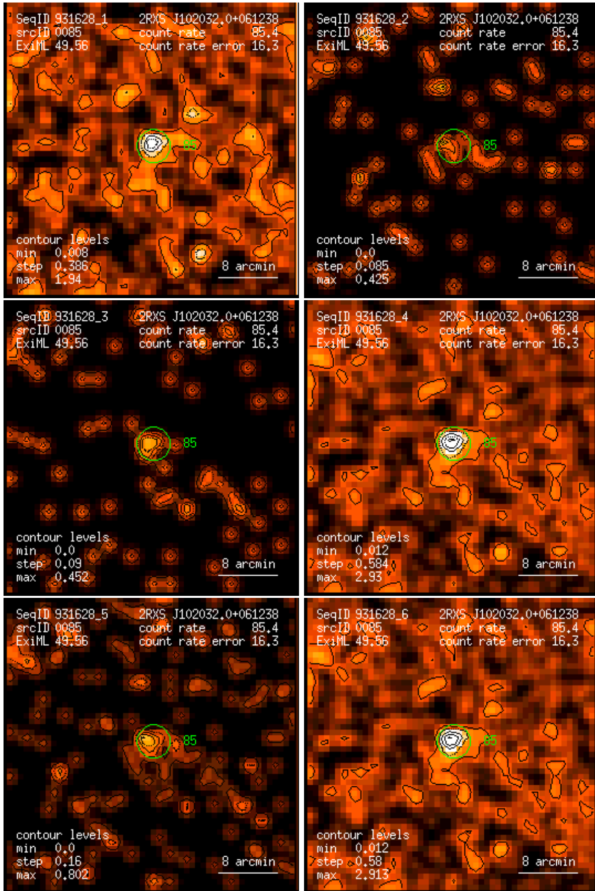
Figure 85: RASS 931628: detection 0085: band rate images, Gaussian filter: (1) PSPC channels 11 – 41, (2) 52 – 90, (3) 91 – 201, (4) 11 – 235, (5) 52 – 201, (6) 11 – 201. Broad band rates in counts/ks. Band rate contour levels in counts/ks/arcmin 2 .
