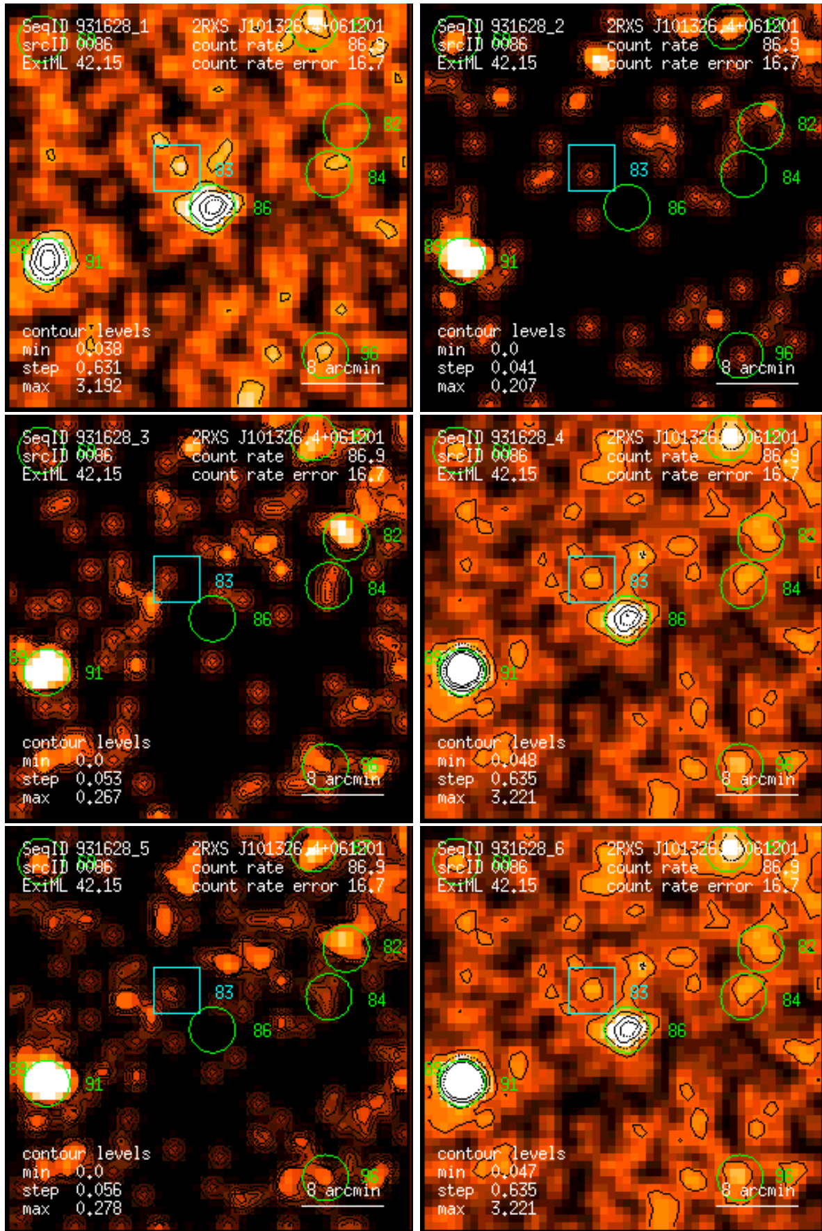
Figure 86: RASS 931628: detection 0086: band rate images, Gaussian filter: (1) PSPC channels 11 – 41, (2) 52 – 90, (3) 91 – 201, (4) 11 – 235, (5) 52 – 201, (6) 11 – 201. Broad band rates in counts/ks. Band rate contour levels in counts/ks/arcmin 2 .
