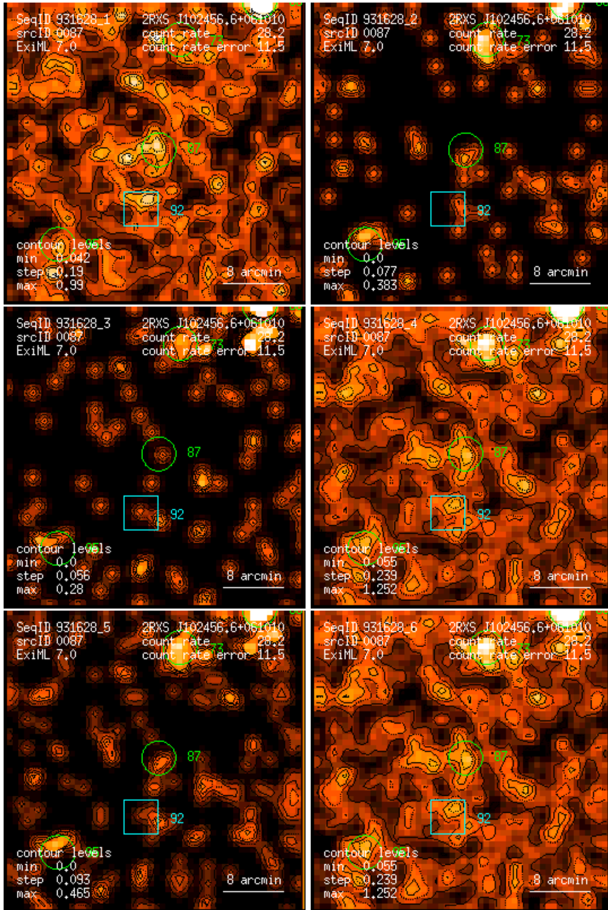
Figure 87: RASS 931628: detection 0087: band rate images, Gaussian filter: (1) PSPC channels 11 – 41, (2) 52 – 90, (3) 91 – 201, (4) 11 – 235, (5) 52 – 201, (6) 11 – 201. Broad band rates in counts/ks. Band rate contour levels in counts/ks/arcmin 2 .
