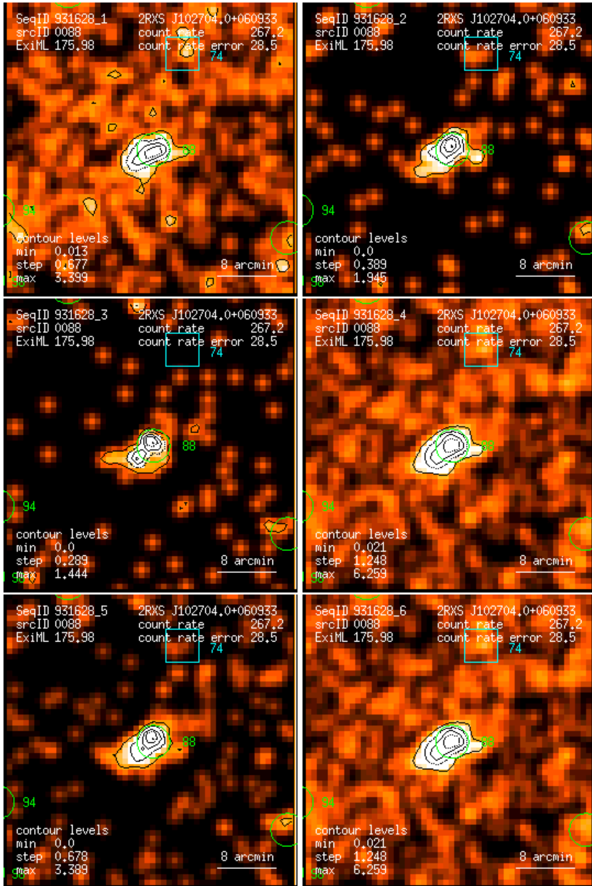
Figure 88: RASS 931628: detection 0088: band rate images, Gaussian filter: (1) PSPC channels 11 – 41, (2) 52 – 90, (3) 91 – 201, (4) 11 – 235, (5) 52 – 201, (6) 11 – 201. Broad band rates in counts/ks. Band rate contour levels in counts/ks/arcmin 2 .
