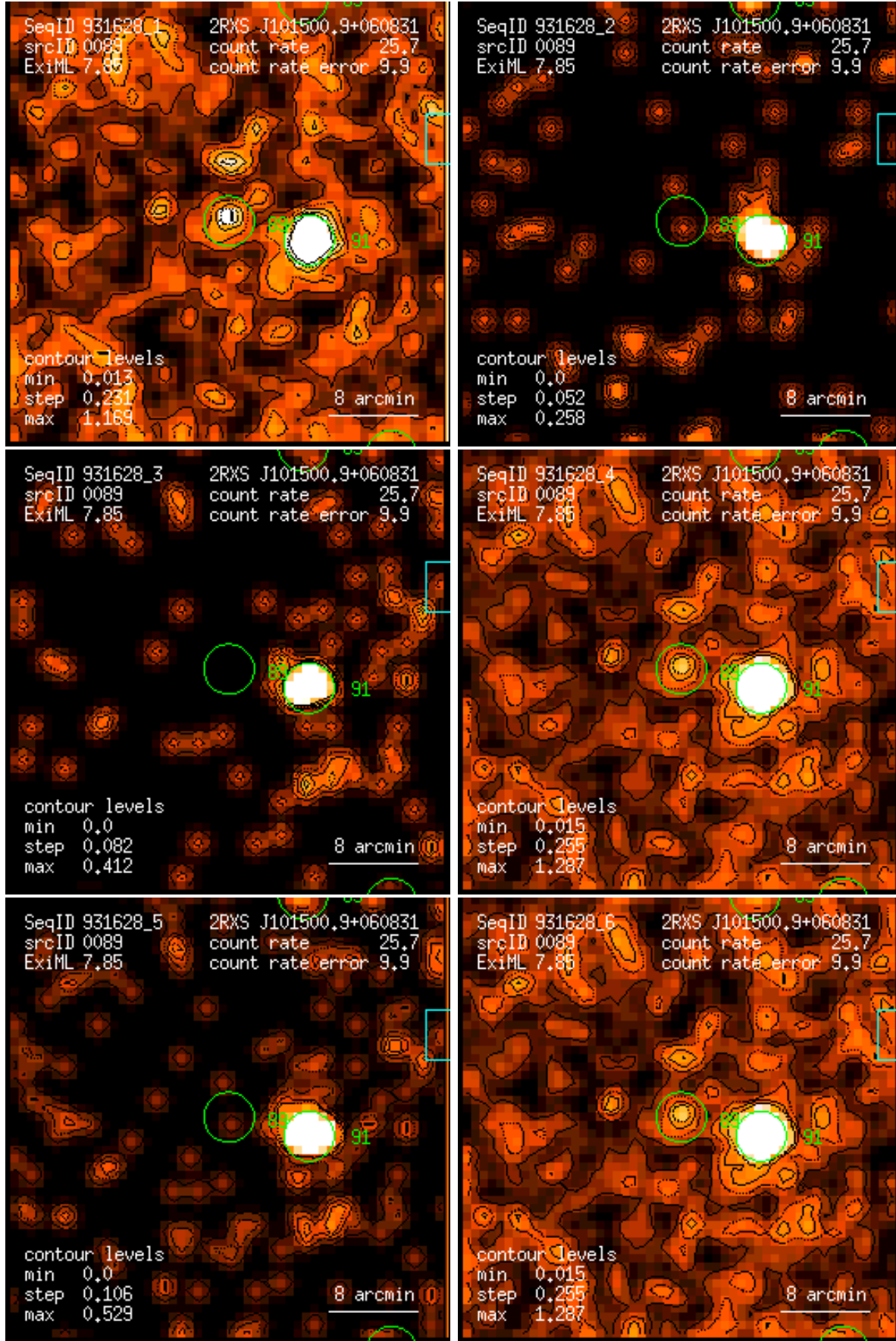
Figure 89: RASS 931628: detection 0089: band rate images, Gaussian filter: (1) PSPC channels 11 – 41, (2) 52 – 90, (3) 91 – 201, (4) 11 – 235, (5) 52 – 201, (6) 11 – 201. Broad band rates in counts/ks. Band rate contour levels in counts/ks/arcmin 2 .
