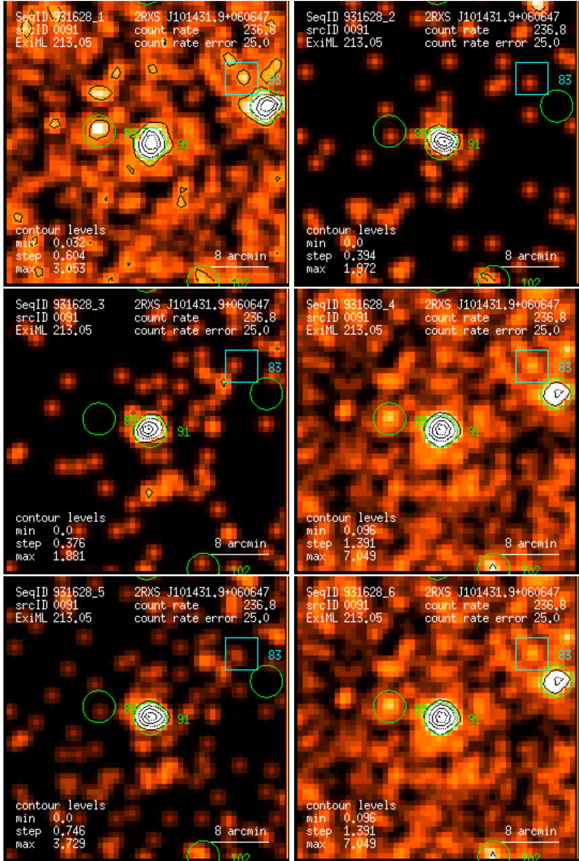
Figure 91: RASS 931628: detection 0091: band rate images, Gaussian filter: (1) PSPC channels 11 – 41, (2) 52 – 90, (3) 91 – 201, (4) 11 – 235, (5) 52 – 201, (6) 11 – 201. Broad band rates in counts/ks. Band rate contour levels in counts/ks/arcmin 2 .
