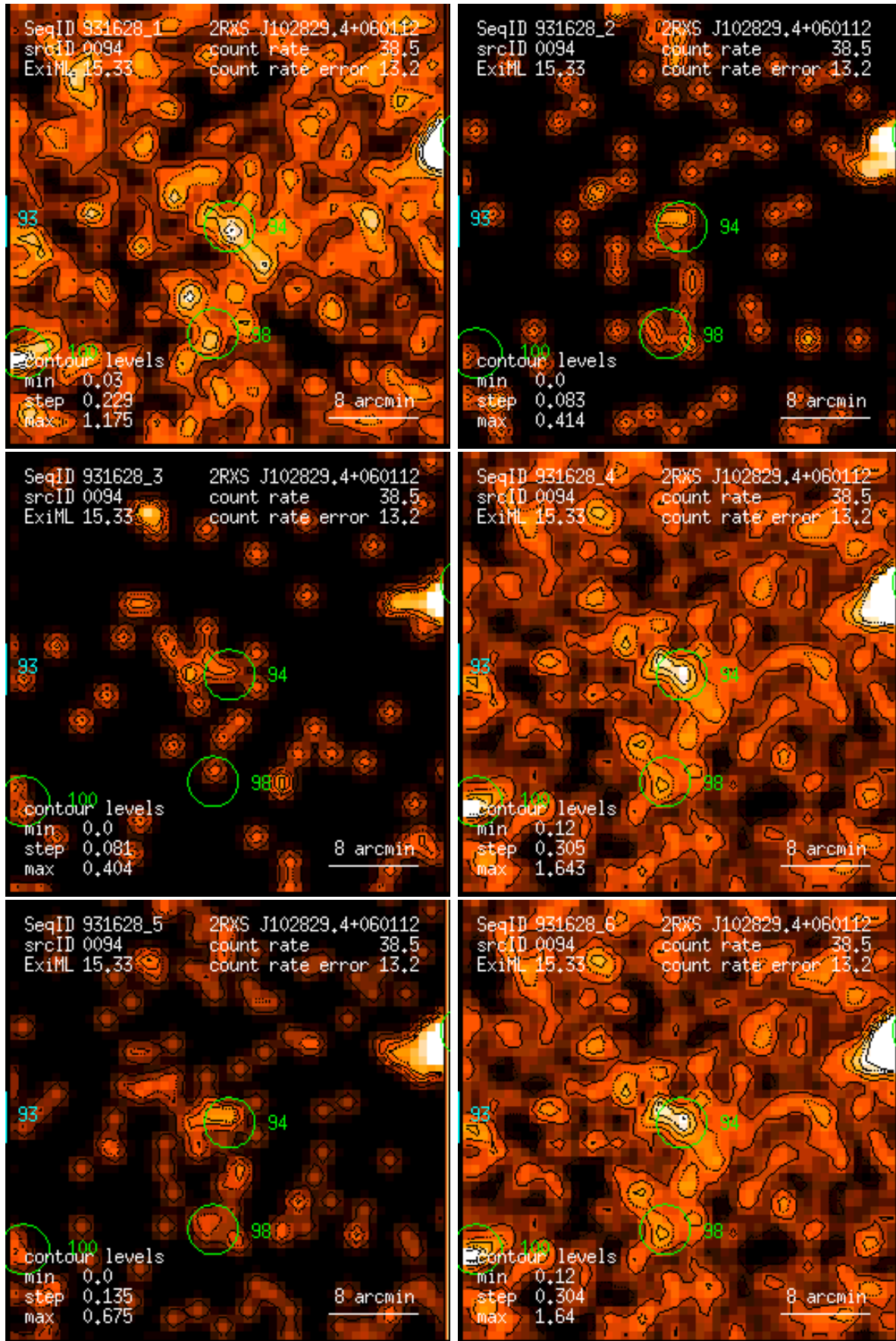
Figure 94: RASS 931628: detection 0094: band rate images, Gaussian filter: (1) PSPC channels 11 – 41, (2) 52 – 90, (3) 91 – 201, (4) 11 – 235, (5) 52 – 201, (6) 11 – 201. Broad band rates in counts/ks. Band rate contour levels in counts/ks/arcmin 2 .
