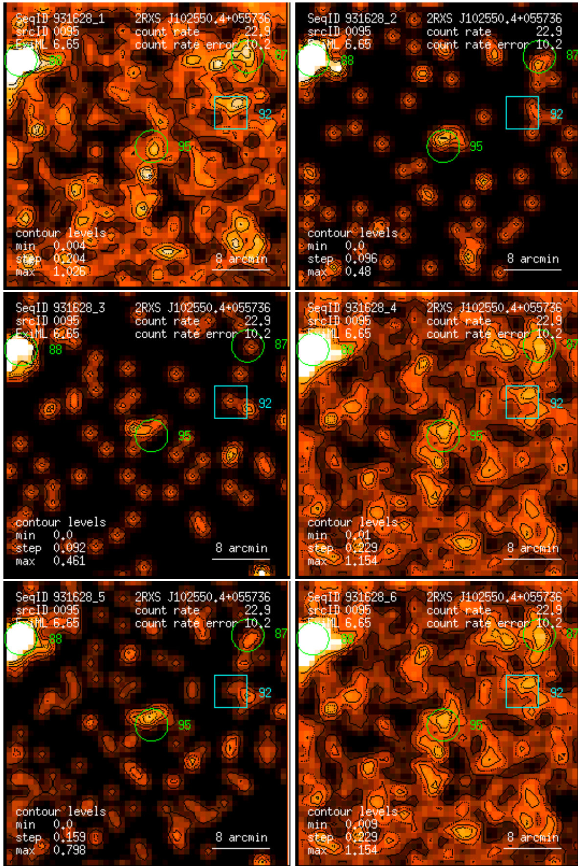
Figure 95: RASS 931628: detection 0095: band rate images, Gaussian filter: (1) PSPC channels 11 – 41, (2) 52 – 90, (3) 91 – 201, (4) 11 – 235, (5) 52 – 201, (6) 11 – 201. Broad band rates in counts/ks. Band rate contour levels in counts/ks/arcmin 2 .
