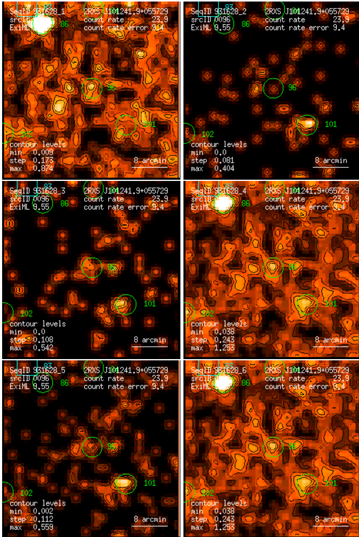
Figure 96: RASS 931628: detection 0096: band rate images, Gaussian filter: (1) PSPC channels 11 – 41, (2) 52 – 90, (3) 91 – 201, (4) 11 – 235, (5) 52 – 201, (6) 11 – 201. Broad band rates in counts/ks. Band rate contour levels in counts/ks/arcmin 2 .
