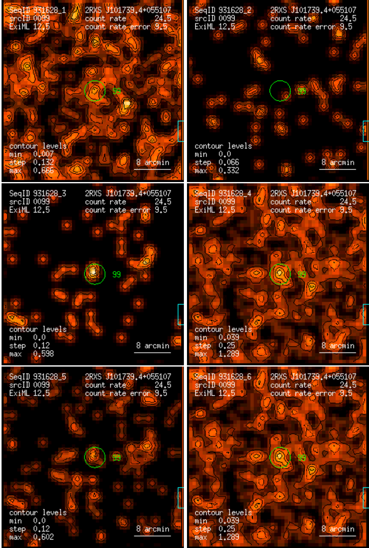
Figure 99: RASS 931628: detection 0099: band rate images, Gaussian filter: (1) PSPC channels 11 – 41, (2) 52 – 90, (3) 91 – 201, (4) 11 – 235, (5) 52 – 201, (6) 11 – 201. Broad band rates in counts/ks. Band rate contour levels in counts/ks/arcmin 2 .
