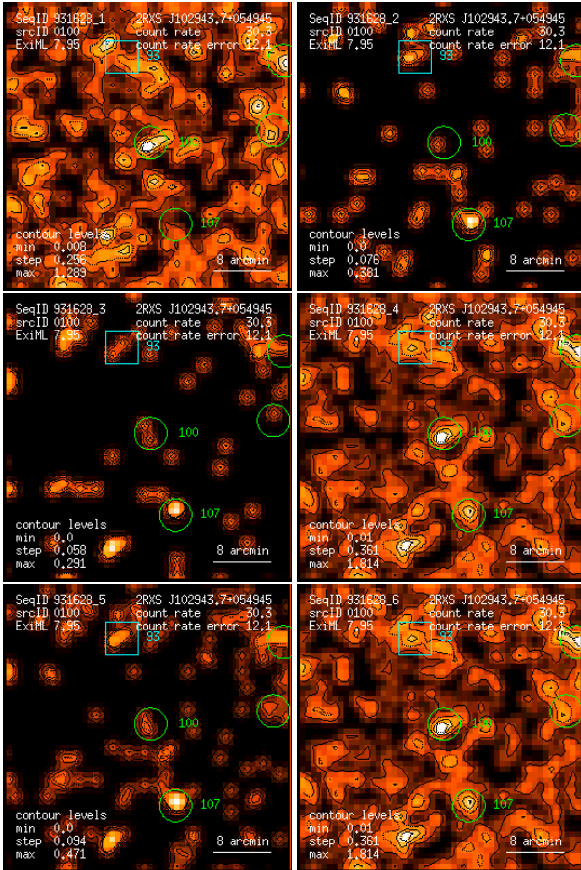
Figure 100: RASS 931628: detection 0100: band rate images, Gaussian filter: (1) PSPC channels 11 – 41, (2) 52 – 90, (3) 91 – 201, (4) 11 – 235, (5) 52 – 201, (6) 11 – 201. Broad band rates in counts/ks. Band rate contour levels in counts/ks/arcmin 2 .
