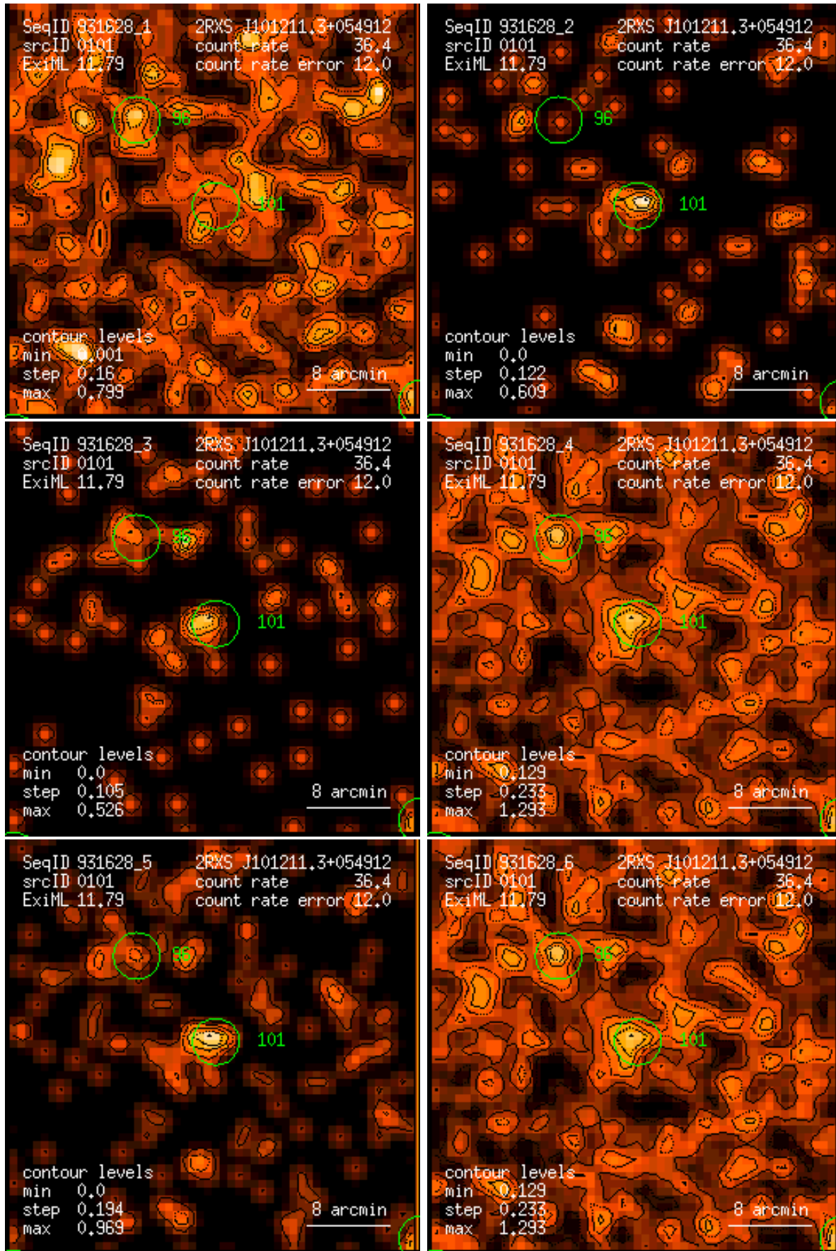
Figure 101: RASS 931628: detection 0101: band rate images, Gaussian filter: (1) PSPC channels 11 – 41, (2) 52 – 90, (3) 91 – 201, (4) 11 – 235, (5) 52 – 201, (6) 11 – 201. Broad band rates in counts/ks. Band rate contour levels in counts/ks/arcmin 2 .
