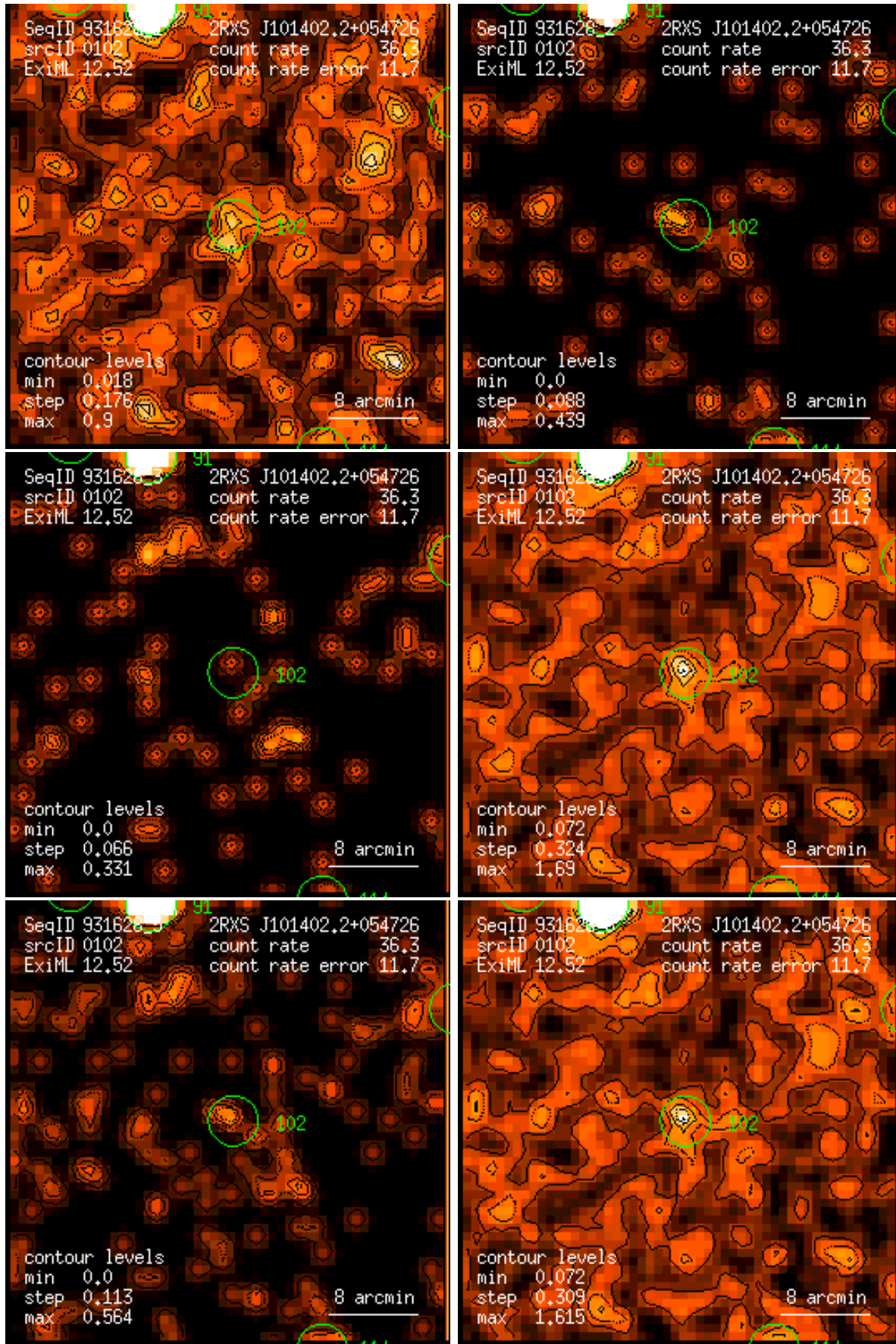
Figure 102: RASS 931628: detection 0102: band rate images, Gaussian filter: (1) PSPC channels 11 – 41, (2) 52 – 90, (3) 91 – 201, (4) 11 – 235, (5) 52 – 201, (6) 11 – 201. Broad band rates in counts/ks. Band rate contour levels in counts/ks/arcmin 2 .
