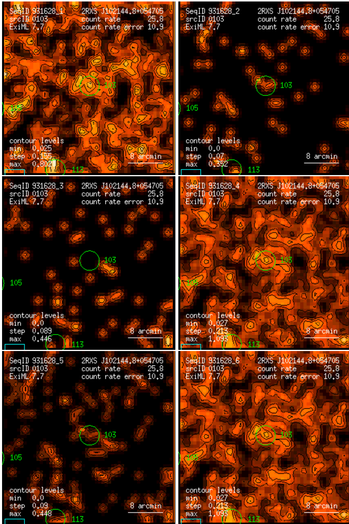
Figure 103: RASS 931628: detection 0103: band rate images, Gaussian filter: (1) PSPC channels 11 – 41, (2) 52 – 90, (3) 91 – 201, (4) 11 – 235, (5) 52 – 201, (6) 11 – 201. Broad band rates in counts/ks. Band rate contour levels in counts/ks/arcmin 2 .
