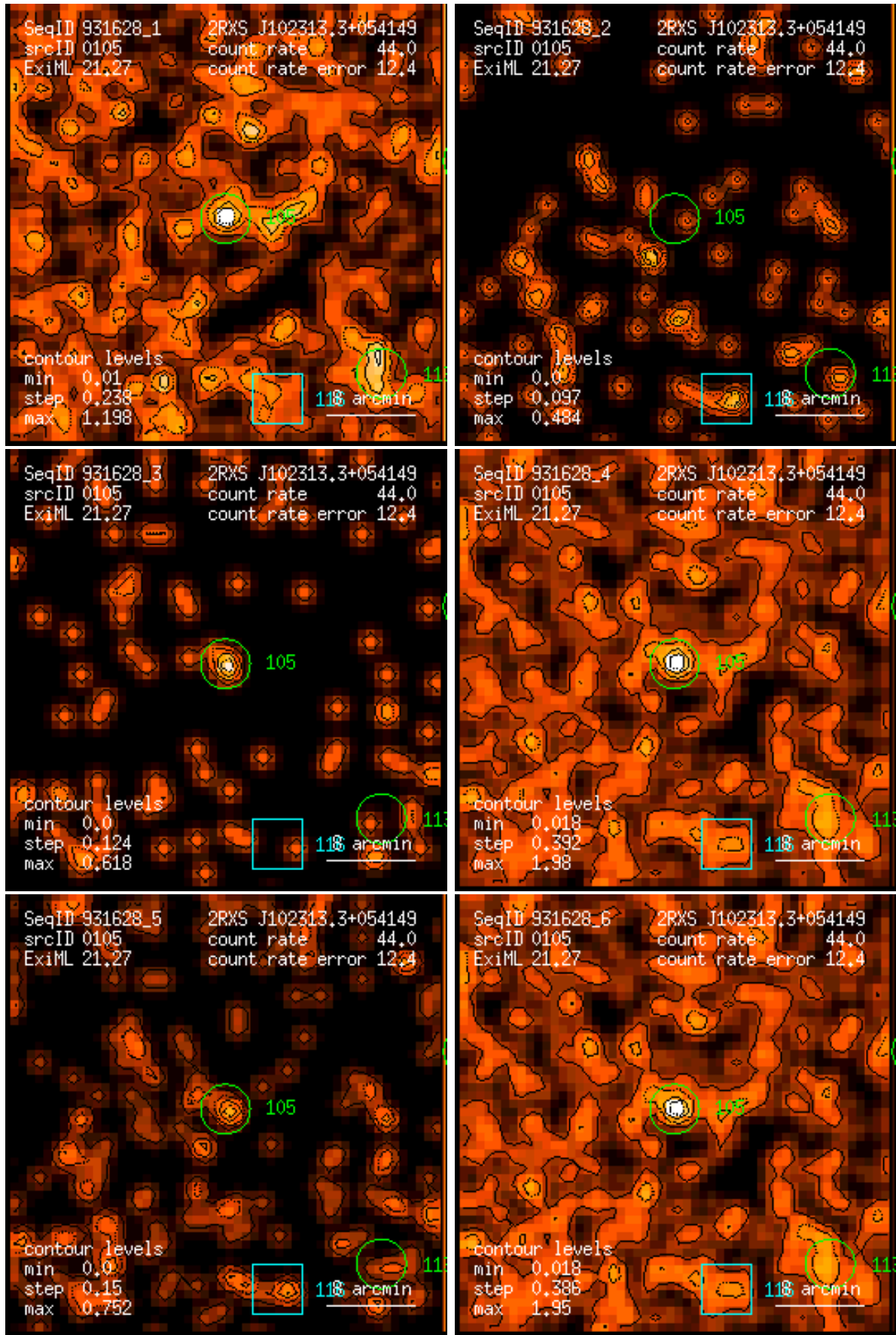
Figure 105: RASS 931628: detection 0105: band rate images, Gaussian filter: (1) PSPC channels 11 – 41, (2) 52 – 90, (3) 91 – 201, (4) 11 – 235, (5) 52 – 201, (6) 11 – 201. Broad band rates in counts/ks. Band rate contour levels in counts/ks/arcmin 2 .
