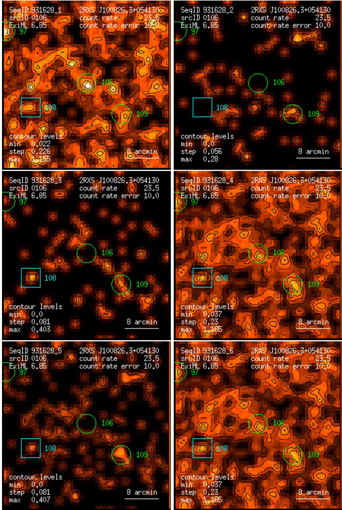
Figure 106: RASS 931628: detection 0106: band rate images, Gaussian filter: (1) PSPC channels 11 – 41, (2) 52 – 90, (3) 91 – 201, (4) 11 – 235, (5) 52 – 201, (6) 11 – 201. Broad band rates in counts/ks. Band rate contour levels in counts/ks/arcmin 2 .
