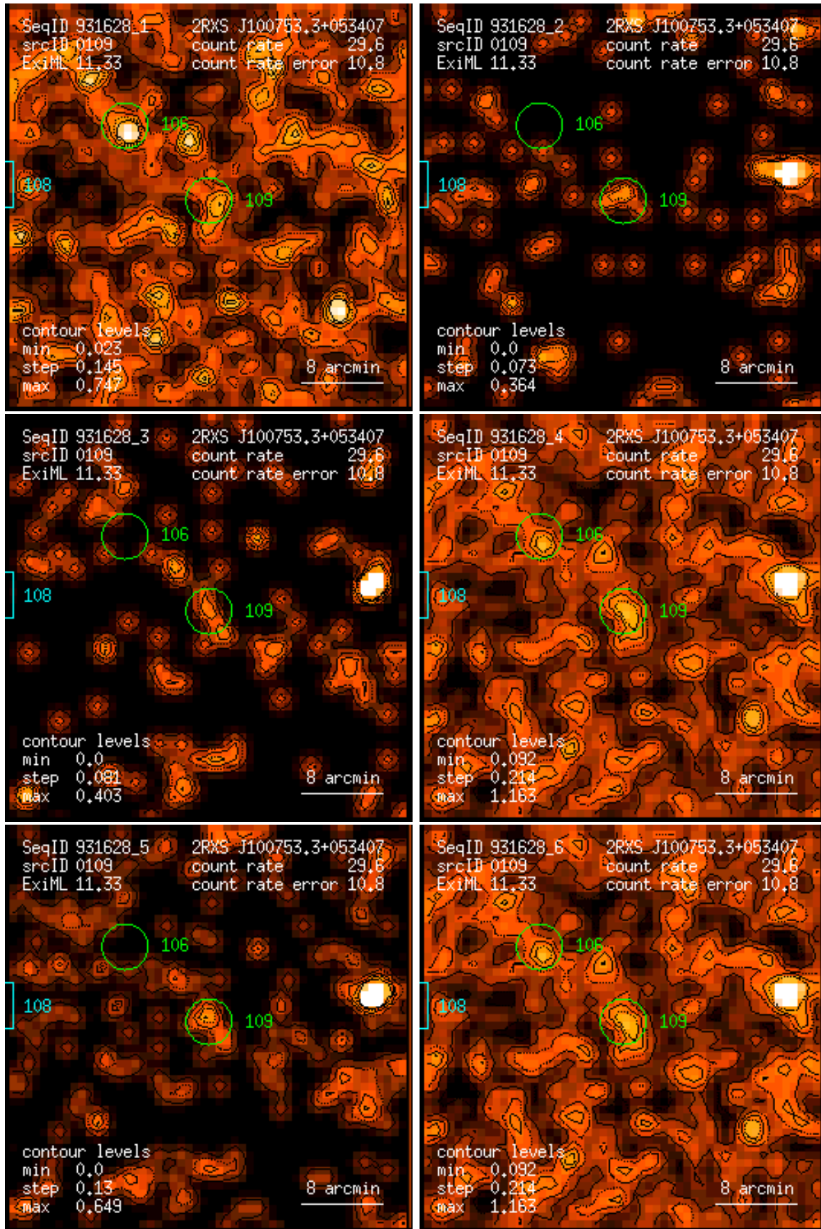
Figure 109: RASS 931628: detection 0109: band rate images, Gaussian filter: (1) PSPC channels 11 – 41, (2) 52 – 90, (3) 91 – 201, (4) 11 – 235, (5) 52 – 201, (6) 11 – 201. Broad band rates in counts/ks. Band rate contour levels in counts/ks/arcmin 2 .
