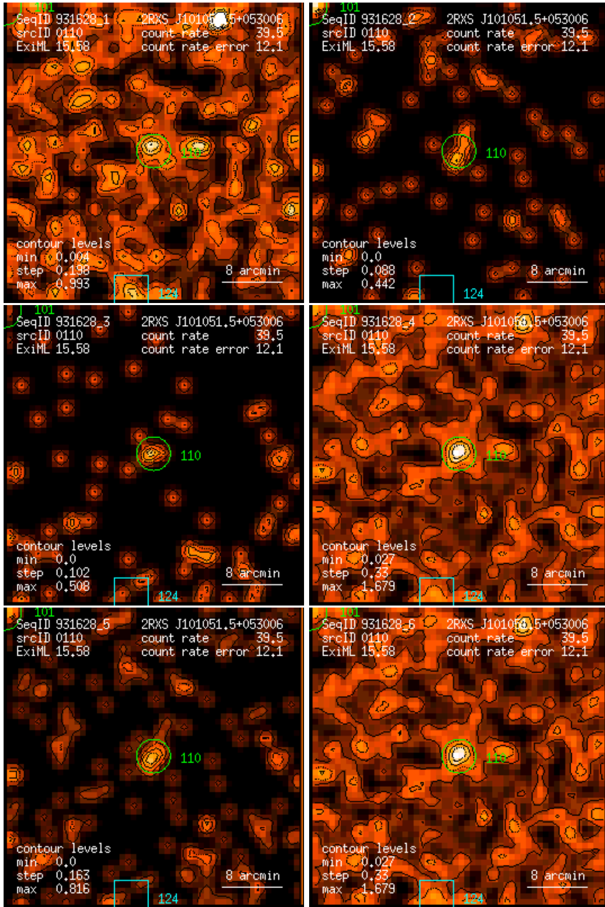
Figure 110: RASS 931628: detection 0110: band rate images, Gaussian filter: (1) PSPC channels 11 – 41, (2) 52 – 90, (3) 91 – 201, (4) 11 – 235, (5) 52 – 201, (6) 11 – 201. Broad band rates in counts/ks. Band rate contour levels in counts/ks/arcmin 2 .
