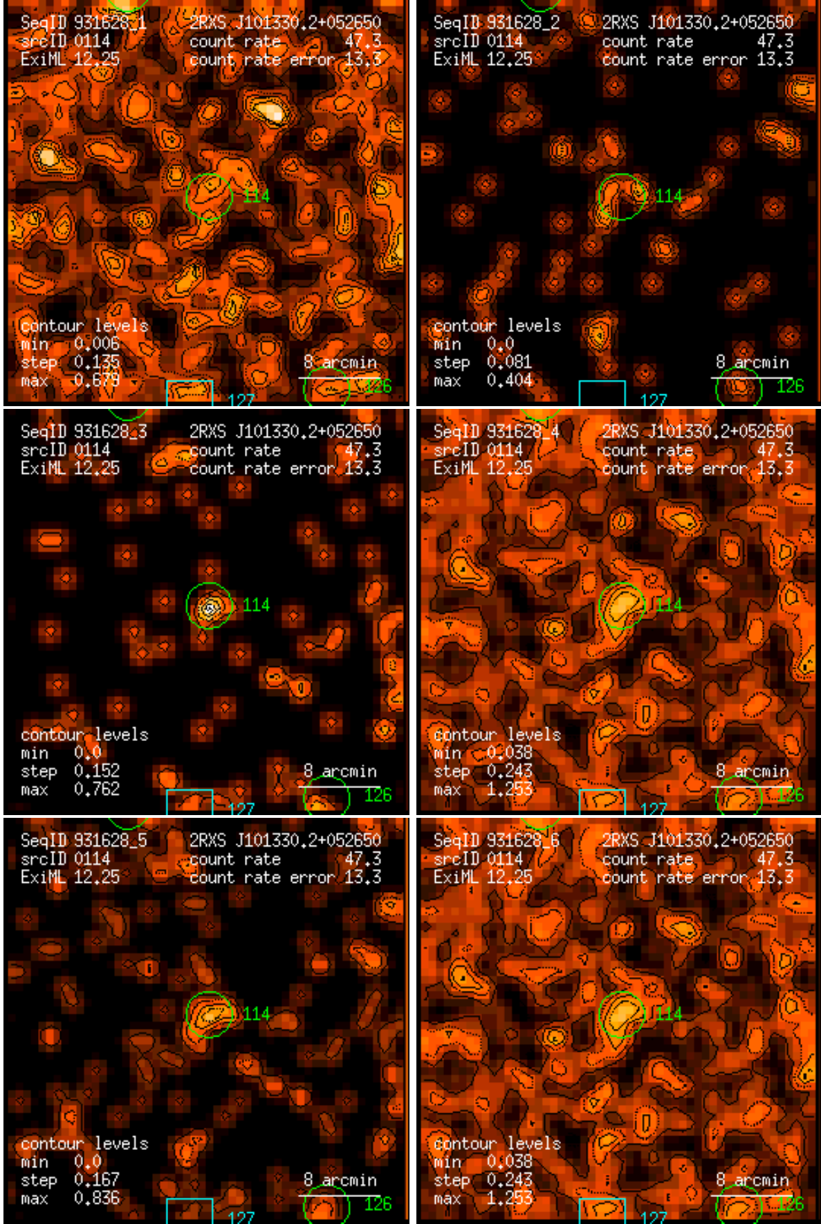
Figure 114: RASS 931628: detection 0114: band rate images, Gaussian filter: (1) PSPC channels 11 – 41, (2) 52 – 90, (3) 91 – 201, (4) 11 – 235, (5) 52 – 201, (6) 11 – 201. Broad band rates in counts/ks. Band rate contour levels in counts/ks/arcmin 2 .
