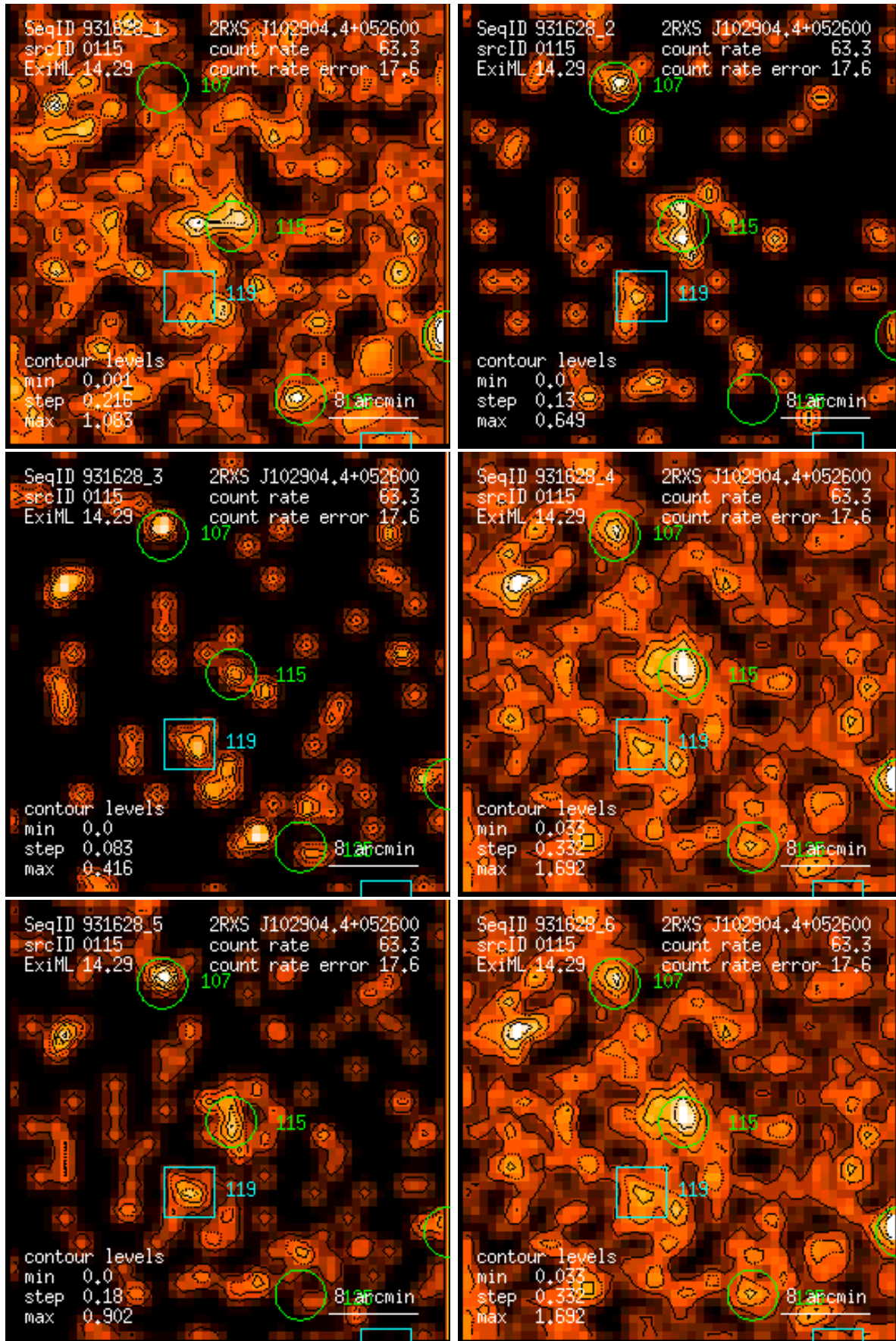
Figure 115: RASS 931628: detection 0115: band rate images, Gaussian filter: (1) PSPC channels 11 – 41, (2) 52 – 90, (3) 91 – 201, (4) 11 – 235, (5) 52 – 201, (6) 11 – 201. Broad band rates in counts/ks. Band rate contour levels in counts/ks/arcmin 2 .
