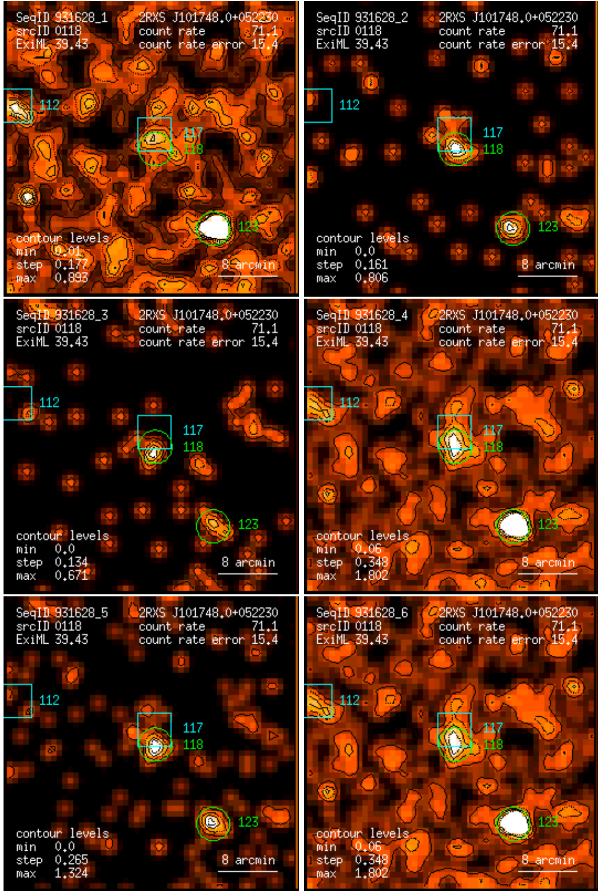
Figure 118: RASS 931628: detection 0118: band rate images, Gaussian filter: (1) PSPC channels 11 – 41, (2) 52 – 90, (3) 91 – 201, (4) 11 – 235, (5) 52 – 201, (6) 11 – 201. Broad band rates in counts/ks. Band rate contour levels in counts/ks/arcmin 2 .
