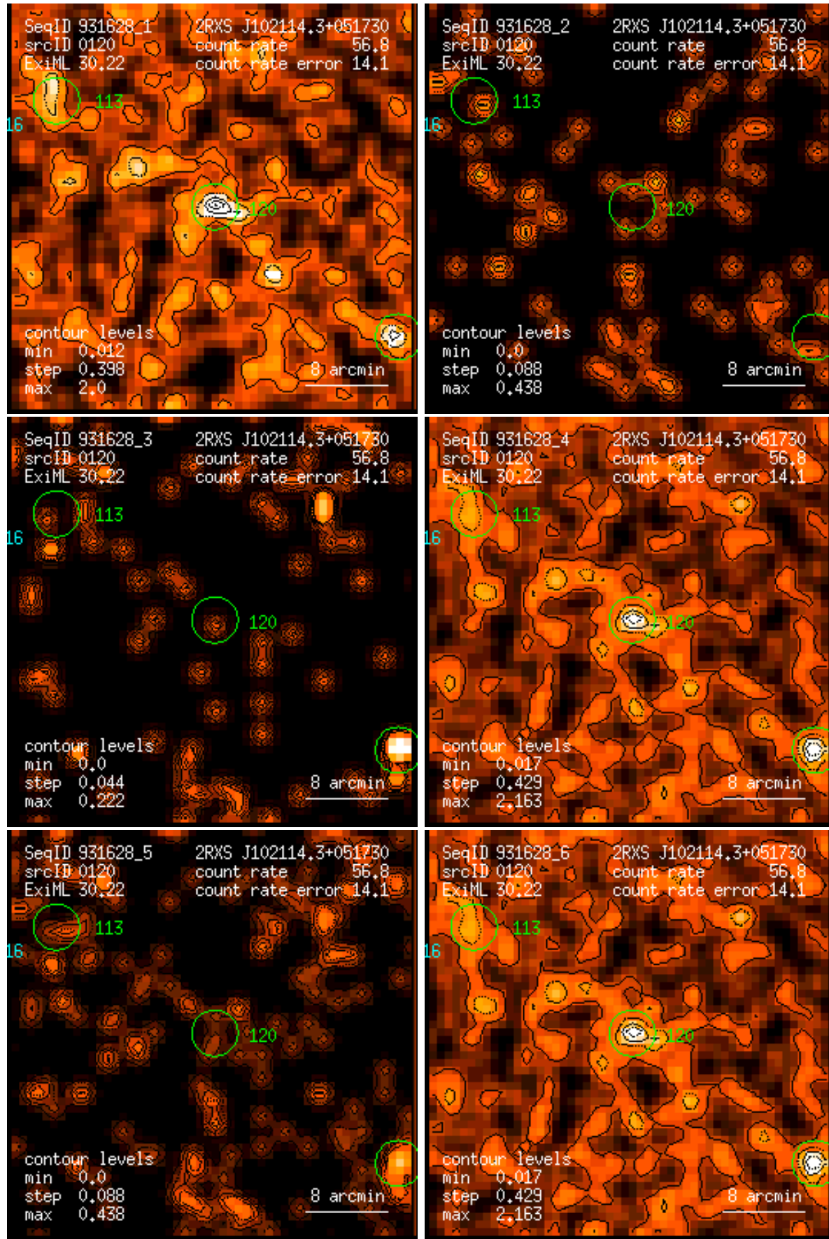
Figure 120: RASS 931628: detection 0120: band rate images, Gaussian filter: (1) PSPC channels 11 – 41, (2) 52 – 90, (3) 91 – 201, (4) 11 – 235, (5) 52 – 201, (6) 11 – 201. Broad band rates in counts/ks. Band rate contour levels in counts/ks/arcmin 2 .
