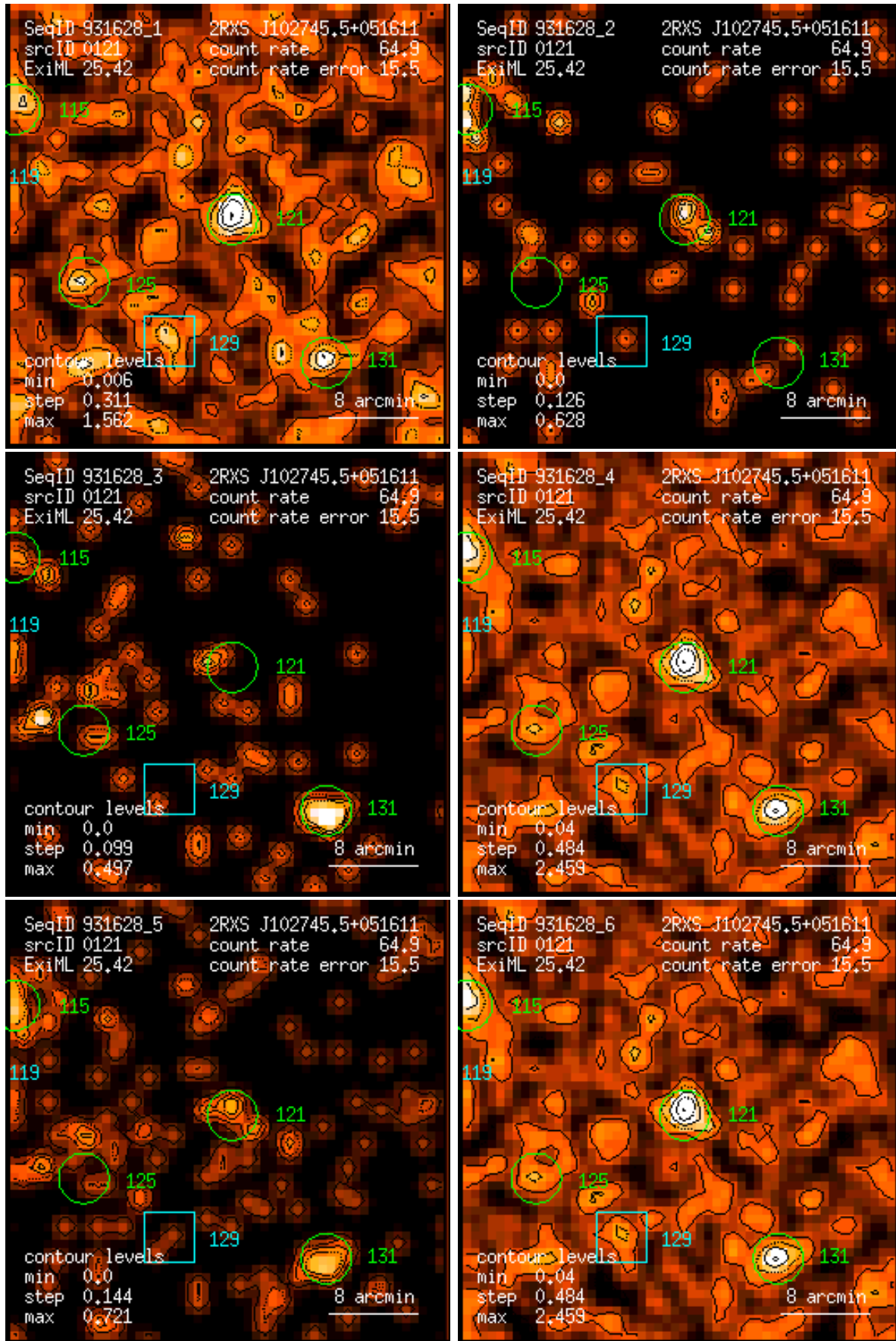
Figure 121: RASS 931628: detection 0121: band rate images, Gaussian filter: (1) PSPC channels 11 – 41, (2) 52 – 90, (3) 91 – 201, (4) 11 – 235, (5) 52 – 201, (6) 11 – 201. Broad band rates in counts/ks. Band rate contour levels in counts/ks/arcmin 2 .
