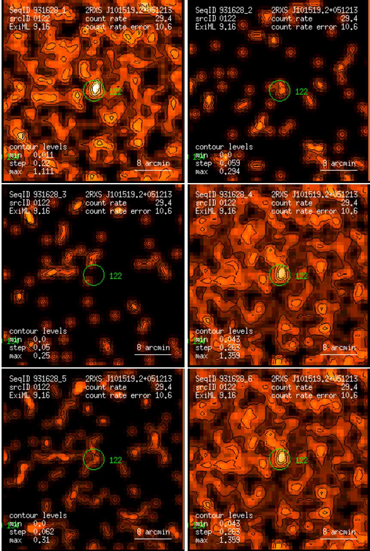
Figure 122: RASS 931628: detection 0122: band rate images, Gaussian filter: (1) PSPC channels 11 – 41, (2) 52 – 90, (3) 91 – 201, (4) 11 – 235, (5) 52 – 201, (6) 11 – 201. Broad band rates in counts/ks. Band rate contour levels in counts/ks/arcmin 2 .
