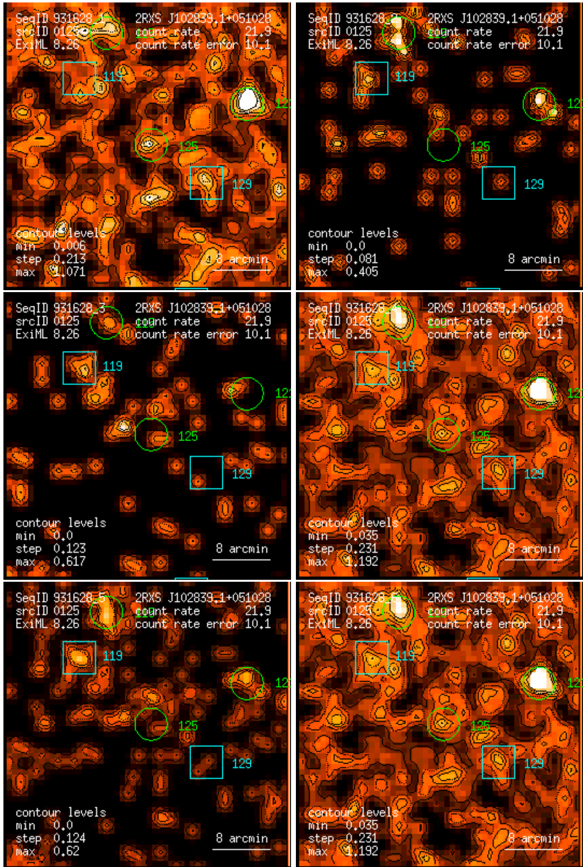
Figure 125: RASS 931628: detection 0125: band rate images, Gaussian filter: (1) PSPC channels 11 – 41, (2) 52 – 90, (3) 91 – 201, (4) 11 – 235, (5) 52 – 201, (6) 11 – 201. Broad band rates in counts/ks. Band rate contour levels in counts/ks/arcmin 2 .
