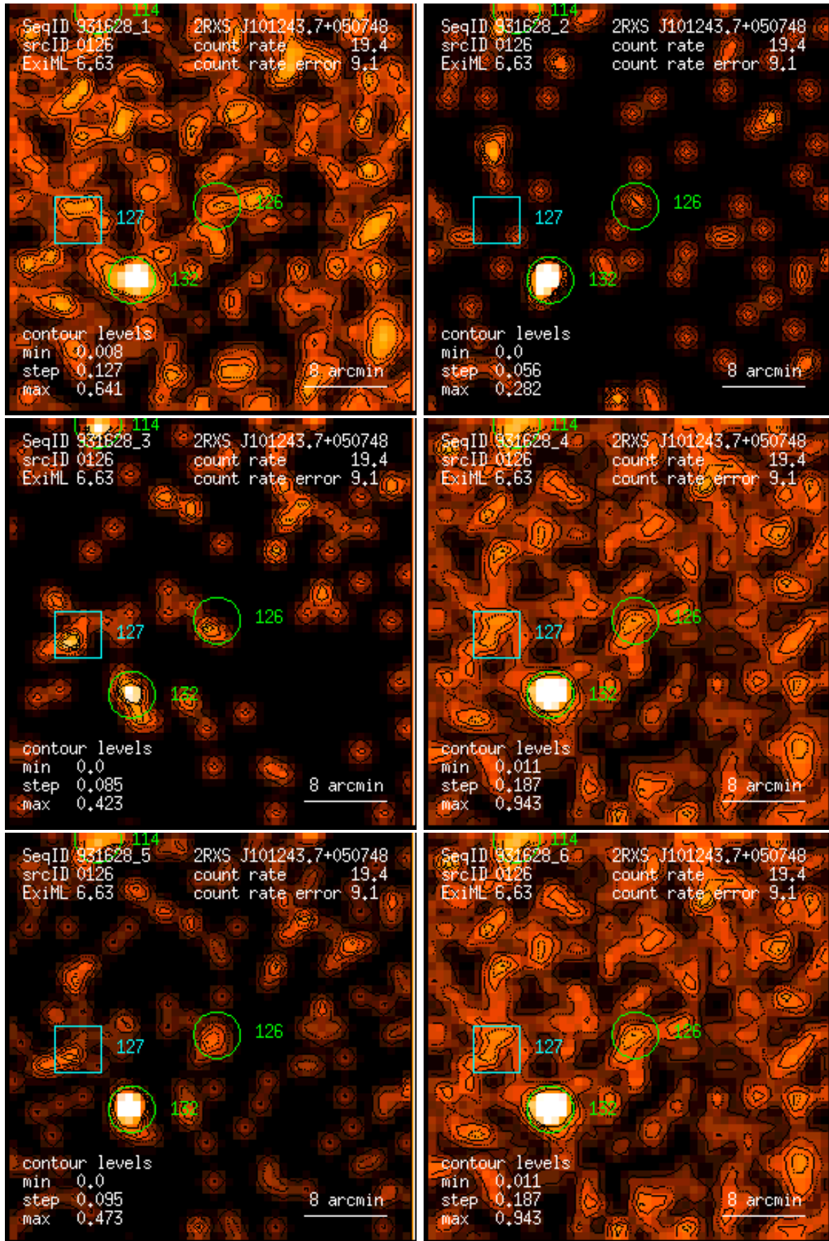
Figure 126: RASS 931628: detection 0126: band rate images, Gaussian filter: (1) PSPC channels 11 – 41, (2) 52 – 90, (3) 91 – 201, (4) 11 – 235, (5) 52 – 201, (6) 11 – 201. Broad band rates in counts/ks. Band rate contour levels in counts/ks/arcmin 2 .
