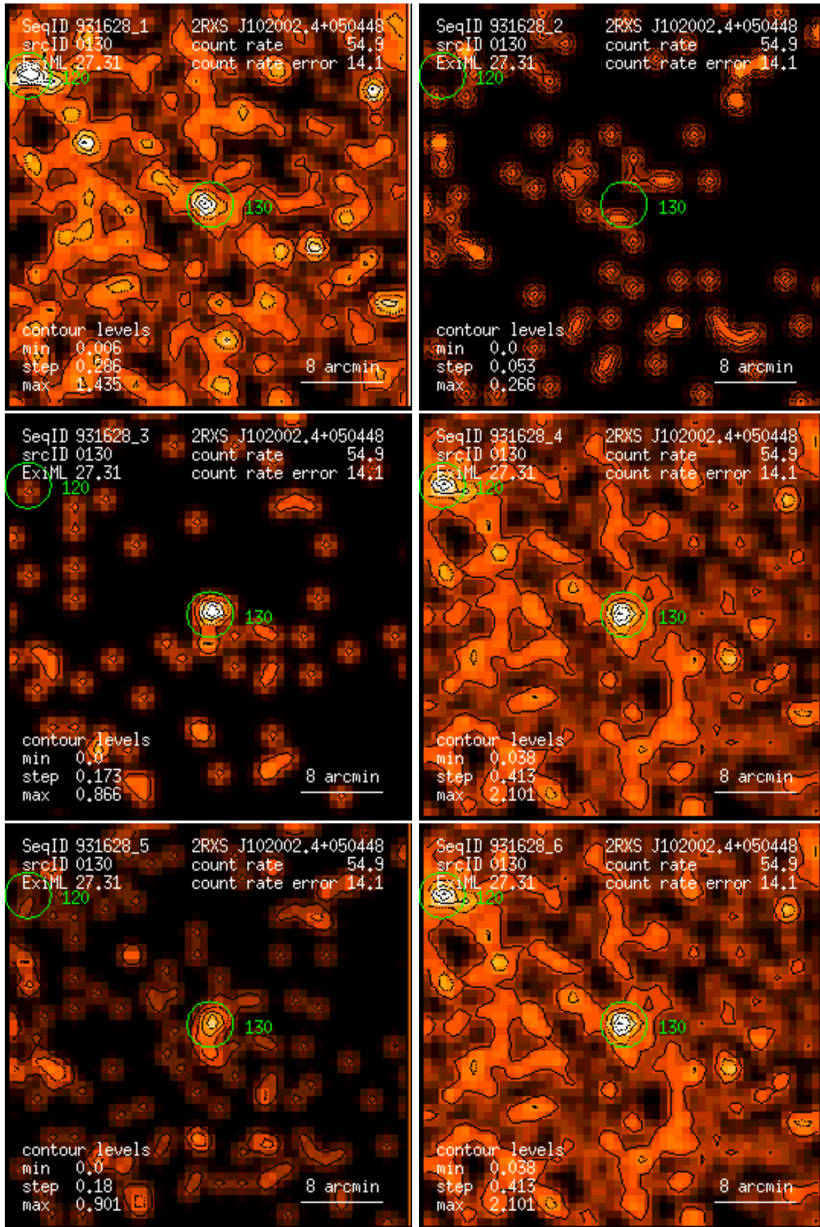
Figure 130: RASS 931628: detection 0130: band rate images, Gaussian filter: (1) PSPC channels 11 – 41, (2) 52 – 90, (3) 91 – 201, (4) 11 – 235, (5) 52 – 201, (6) 11 – 201. Broad band rates in counts/ks. Band rate contour levels in counts/ks/arcmin 2 .
