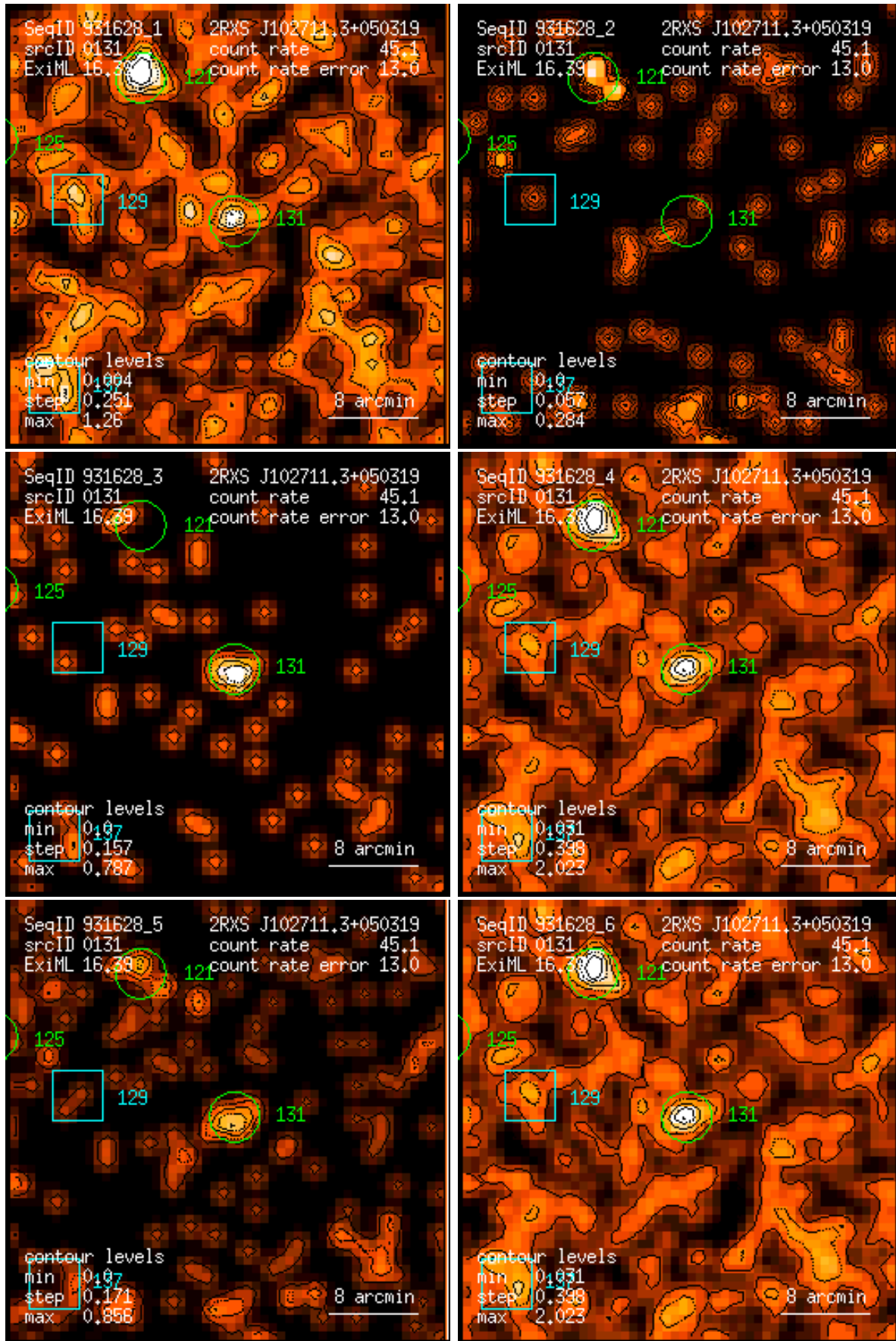
Figure 131: RASS 931628: detection 0131: band rate images, Gaussian filter: (1) PSPC channels 11 – 41, (2) 52 – 90, (3) 91 – 201, (4) 11 – 235, (5) 52 – 201, (6) 11 – 201. Broad band rates in counts/ks. Band rate contour levels in counts/ks/arcmin 2 .
