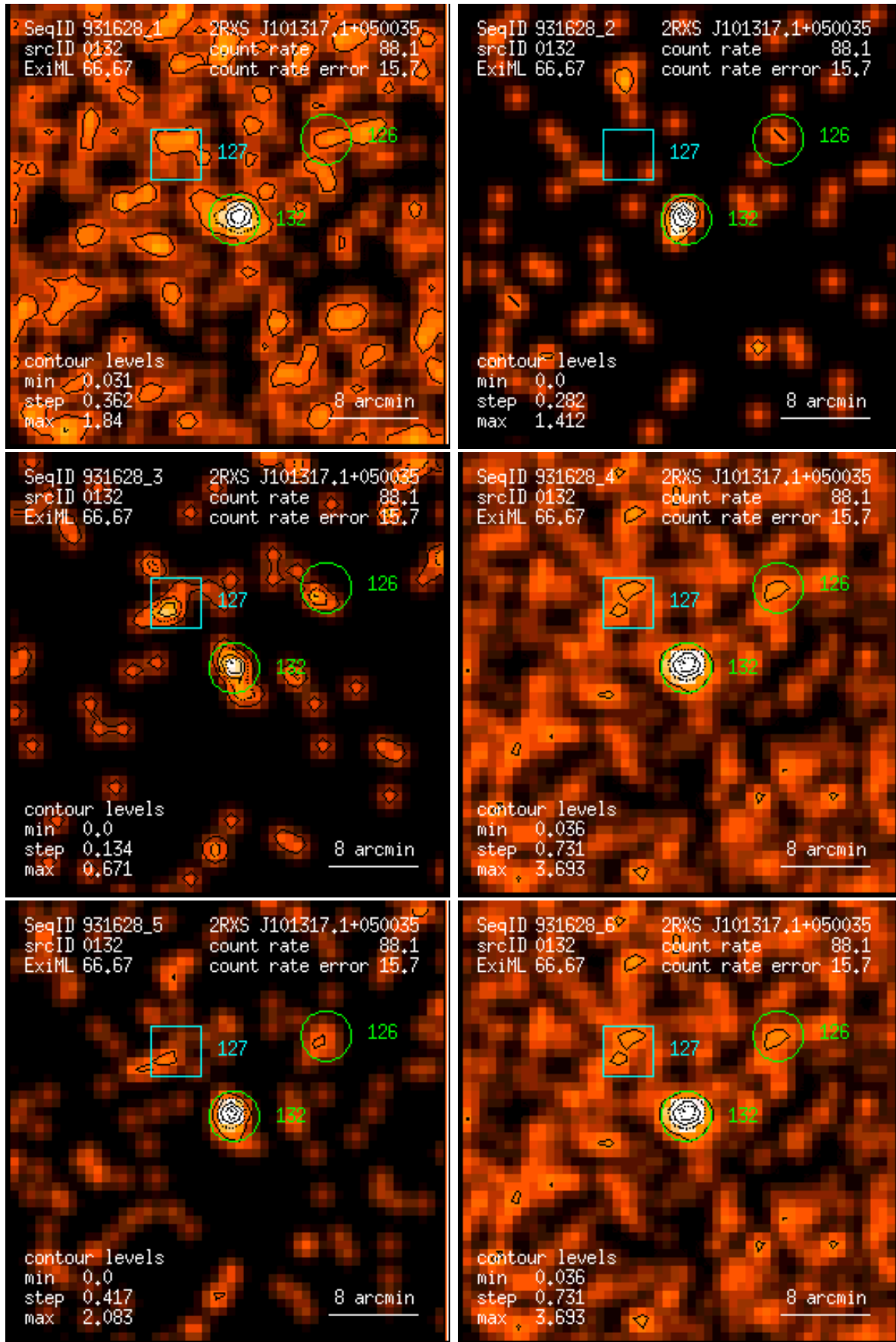
Figure 132: RASS 931628: detection 0132: band rate images, Gaussian filter: (1) PSPC channels 11 – 41, (2) 52 – 90, (3) 91 – 201, (4) 11 – 235, (5) 52 – 201, (6) 11 – 201. Broad band rates in counts/ks. Band rate contour levels in counts/ks/arcmin 2 .
