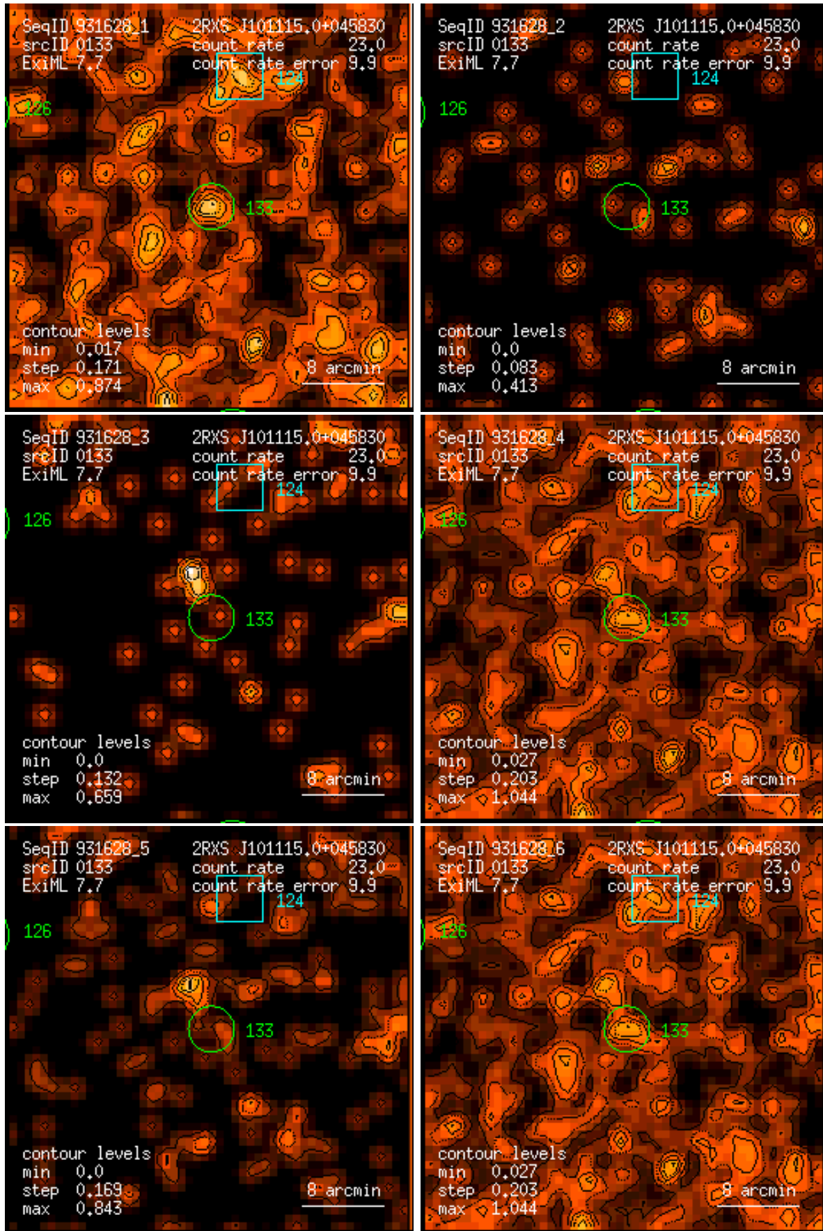
Figure 133: RASS 931628: detection 0133: band rate images, Gaussian filter: (1) PSPC channels 11 – 41, (2) 52 – 90, (3) 91 – 201, (4) 11 – 235, (5) 52 – 201, (6) 11 – 201. Broad band rates in counts/ks. Band rate contour levels in counts/ks/arcmin 2 .
