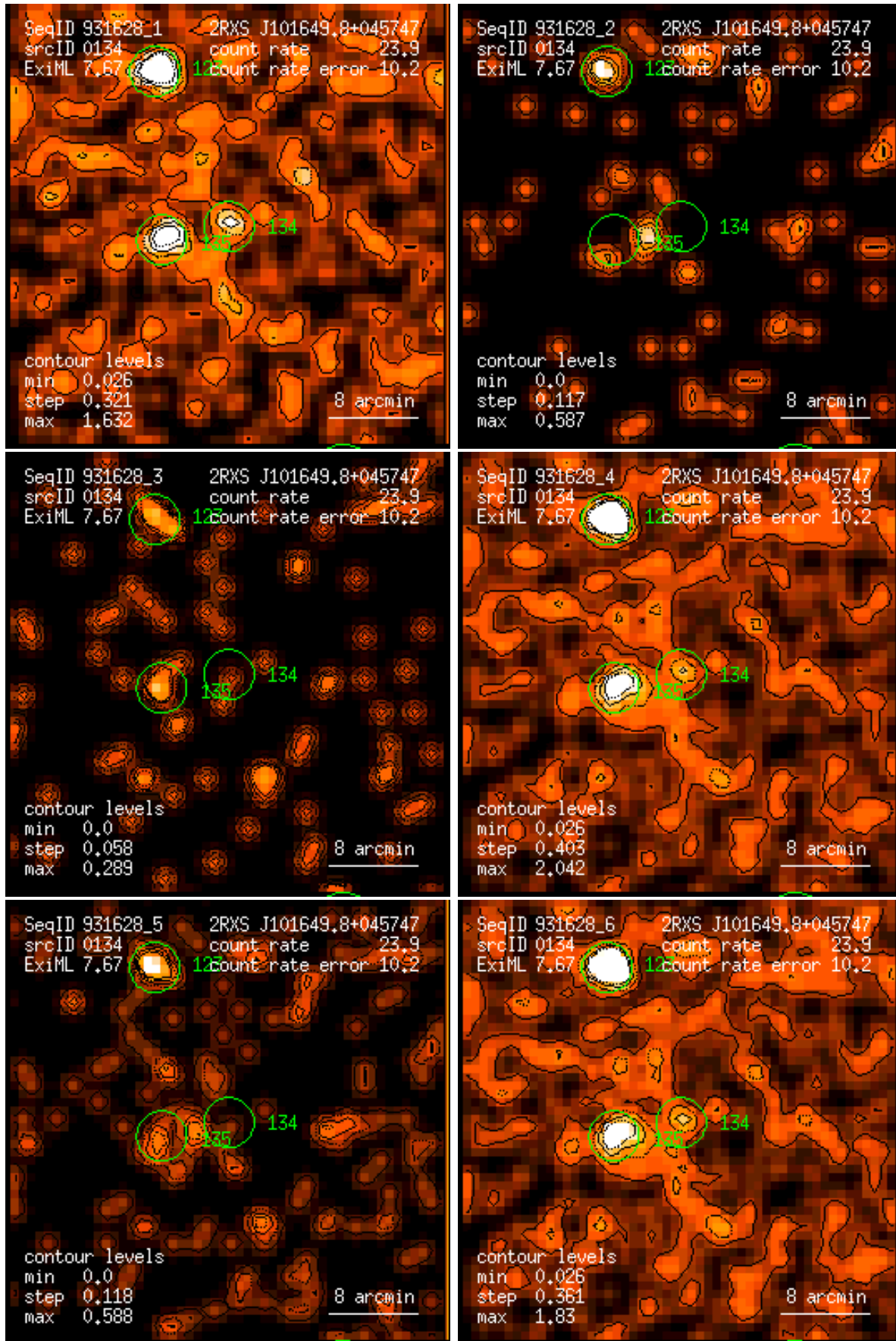
Figure 134: RASS 931628: detection 0134: band rate images, Gaussian filter: (1) PSPC channels 11 – 41, (2) 52 – 90, (3) 91 – 201, (4) 11 – 235, (5) 52 – 201, (6) 11 – 201. Broad band rates in counts/ks. Band rate contour levels in counts/ks/arcmin 2 .
