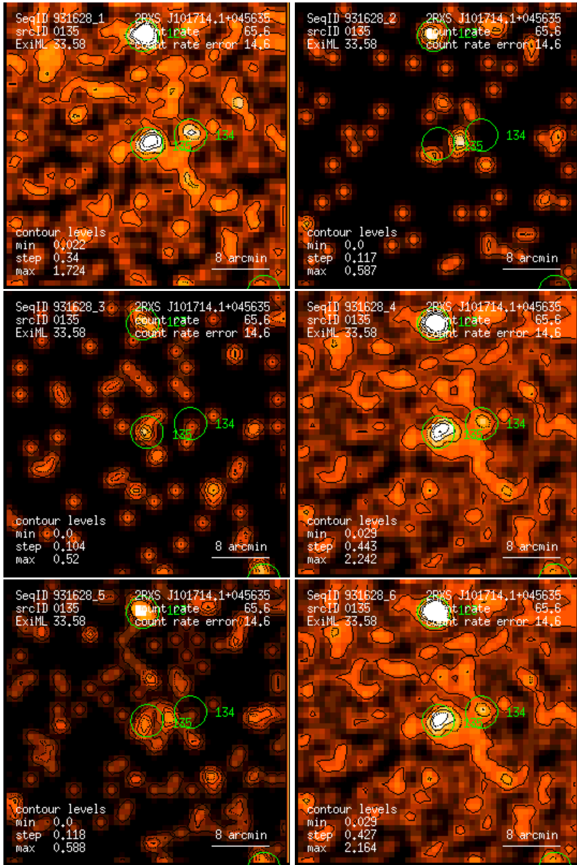
Figure 135: RASS 931628: detection 0135: band rate images, Gaussian filter: (1) PSPC channels 11 – 41, (2) 52 – 90, (3) 91 – 201, (4) 11 – 235, (5) 52 – 201, (6) 11 – 201. Broad band rates in counts/ks. Band rate contour levels in counts/ks/arcmin 2 .
