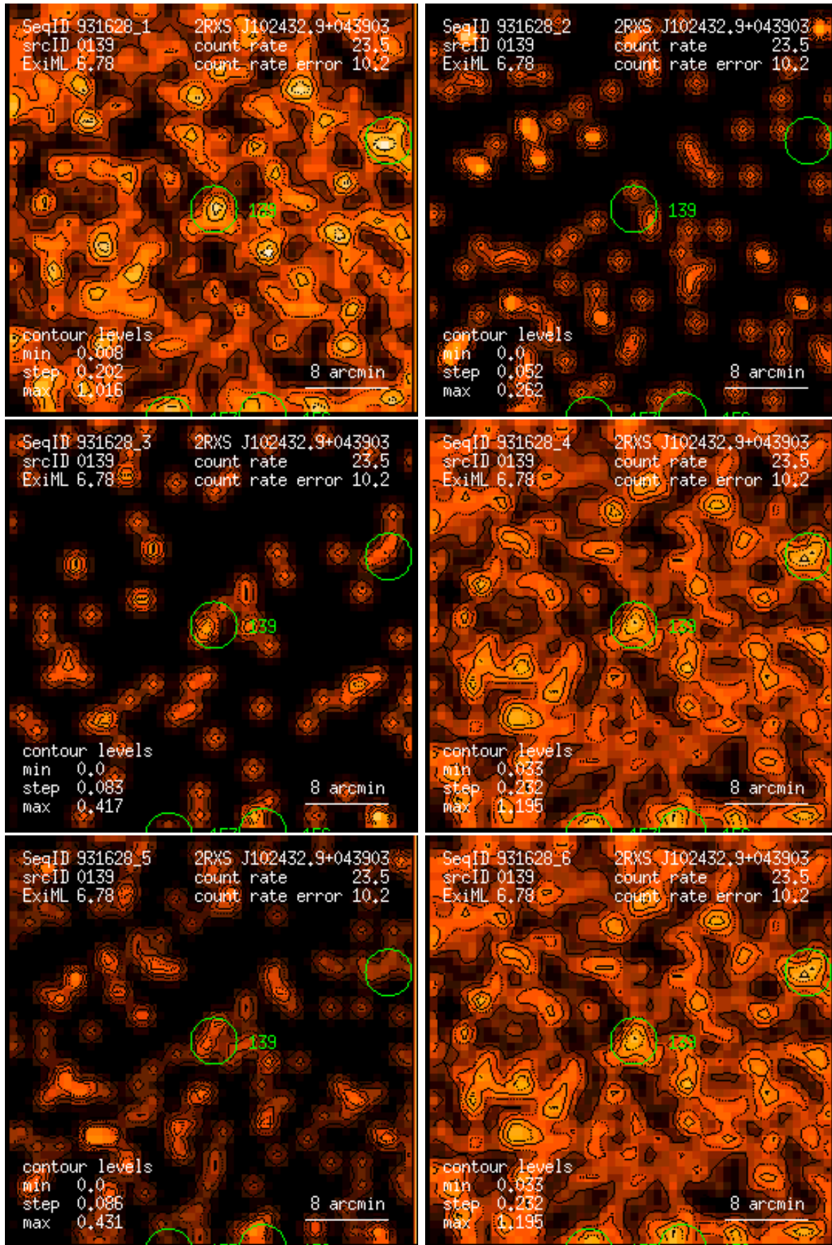
Figure 139: RASS 931628: detection 0139: band rate images, Gaussian filter: (1) PSPC channels 11 – 41, (2) 52 – 90, (3) 91 – 201, (4) 11 – 235, (5) 52 – 201, (6) 11 – 201. Broad band rates in counts/ks. Band rate contour levels in counts/ks/arcmin 2 .
