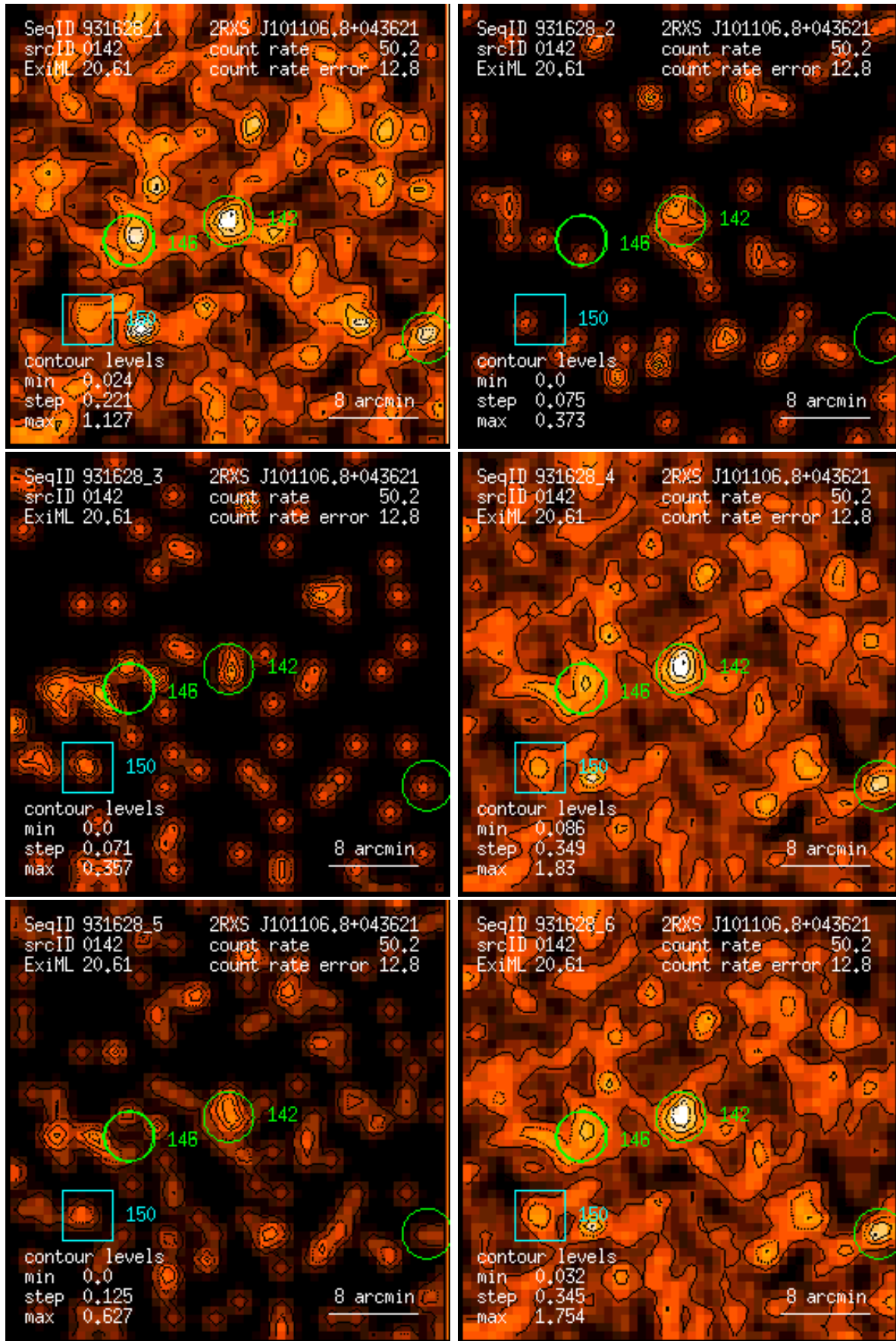
Figure 142: RASS 931628: detection 0142: band rate images, Gaussian filter: (1) PSPC channels 11 – 41, (2) 52 – 90, (3) 91 – 201, (4) 11 – 235, (5) 52 – 201, (6) 11 – 201. Broad band rates in counts/ks. Band rate contour levels in counts/ks/arcmin 2 .
